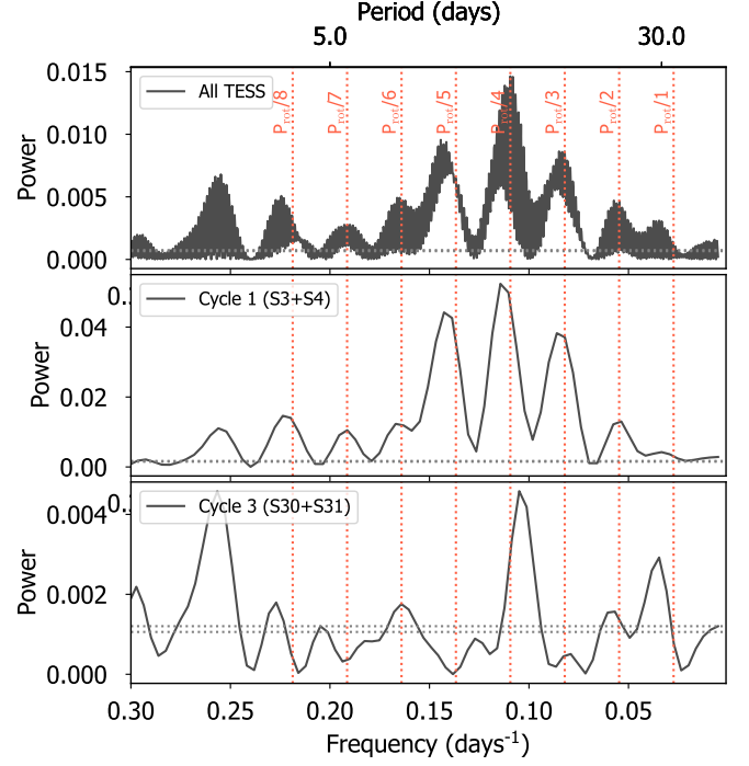
Fig. A.3. TESS light curve generalized Lomb-Scargle periodogram. Upper panel: GLSP using the full TESS dataset. Middle panel: GLSP using TESS data from Cycle 1, including sector 3 and 4. Lower panel: GLSP using TESS data from Cycle 3, including sector 30 and 31. In all panels, we highlight the first eight harmonics of the fundamental frequency corresponding to the expected rotation period of the star according to our RV analysis (see Sect. 3) and from the expected value from the empirical relations by Suárez Mascareño et al. (2015).
