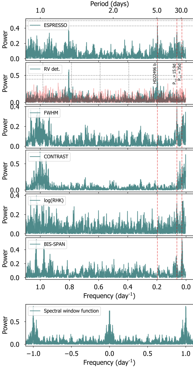
Fig. 2. Periodogram of ESPRESSO time series. From top to bottom: ESPRESSO RV, ESPRESSO RVs after a simple weighted linear detrending with the BIS-SPAN activity indicator (green color) and after removing a Keplerian signal with P = 5.09 days (red), FWHM of the CCF, CONTRAST of the CCF, log(RHK), BIS-SPAN and the window function. The dashed red vertical lines mark the location of the confirmed planet HD 22496 b, the stellar rotation period found by the GP and its alias. In the two upper panels, the dotted horizontal lines mark the 0.1% and 1% false alarm probability levels. In the second panel, the vertical dotted lines mark the first 10 alias periods of the HD 22496 b signal.
