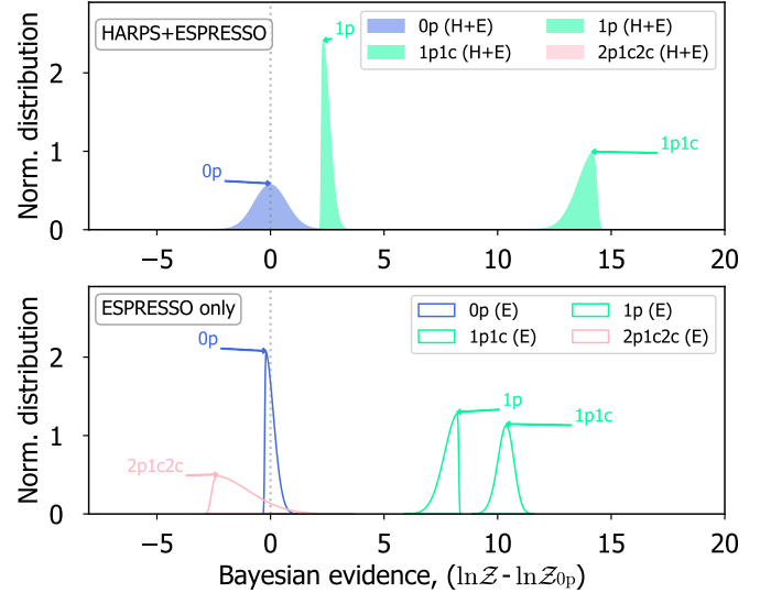
Fig. 3. Distribution of the log-Bayesian evidence for the different models tested using the Gaussian Process approach to account for the stellar activity (see Sect. 3). Filled shaded distributions correspond to the HARPS+ESPRESSO dataset (upper panel) while open distributions correspond to the ESPRESSO standalone dataset (lower panel). The median from the null hypothesis model for each dataset (labelled as 0p) has been subtracted. In the upper panel, the two-planet model ("2p1c2c") has a very low odd ratio, hence lying outside of the plot limits.
