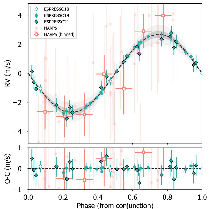
Fig. 4. Radial velocities from HARPS (red) and ESPRESSO (green) phase-folded with the period from planet HD 22496 b. The red open symbols display binned values from HARPS measurements corresponding to 10% of the orbital phase. The median GP model has been subtracted. The bottom panel shows the residuals of the mean model.
