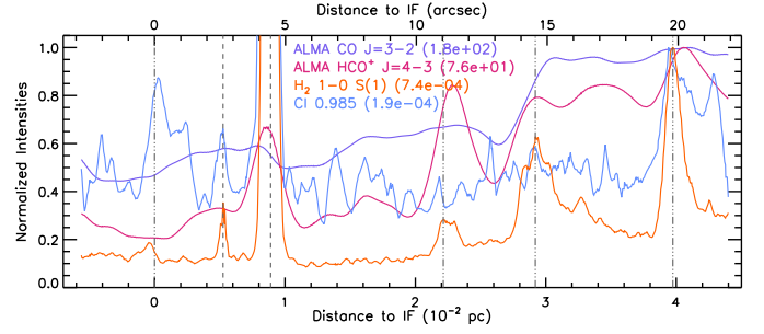
Fig. 20. Comparison of the NIRSpec H 2 1–0 S(1) and C I 0.985 μm observations (in \text{erg cm}^{-2} \text{s}^{-1} \text{sr}^{-1} ) with the ALMA observation at 1'' resolution of the HCO + J=4\text{--}3 line integrated intensity (in \text{K km s}^{-1} ) and the CO J=3\text{--}2 line peak temperatures ( T_{\text{peak}} , Goicoechea et al. 2016). Shown are normalised line intensities as a function of distance to the IF ( 0.228 pc or 113.4'' from \theta^1 Ori C) along a cut crossing the NIRSpec mosaic (see Fig. 1). As the cut is not perpendicular to the IF and distances are given along the cut, a correction factor of \cos(19.58^\circ)=0.942 needs to be applied to obtain a perpendicular distance from the IF. Normalisation factors are listed between brackets for each intensity. No extinction correction is applied. The dash-dot-dot vertical lines indicate the position of the IF, DF 1, DF 2, and DF 3, respectively, from left to right. The dashed vertical lines indicated the location of the proplyds 203–504 (left) and 203–506 (right).
