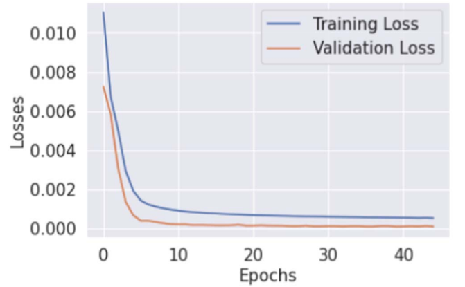
Figure 6. Results of the training process. The orange line shows the loss of the model when it evaluates the validation data, while the blue line represents the loss of the model when it evaluates the training data. When the two losses do not decrease for five epochs, the training algorithm is automatically stopped to prevent overfitting the model on the training data.
