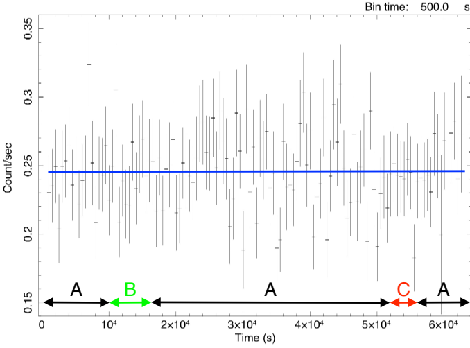
fig. 4. Light curve of the photon count rate in the energy range E = 0.3 –10 keV, from the EPIC-pn observation. The horizontal blue line indicates the average value of the count rate. A, B, and C indicate the time intervals defined in Sect. 5.2.
