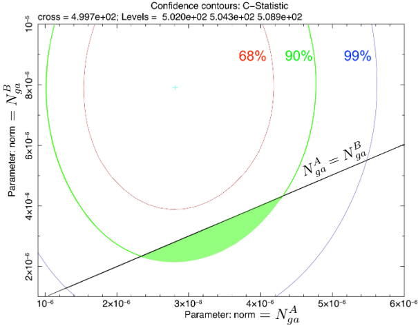
fig. 6. Confidence contours for N_{ga} and N_{ga}^B . The straight black line is drawn in correspondence of N_{ga}^B = N_{ga}^A . The green area is the intersection between the half-plane below the black line and the region contained inside the 90% contour.
