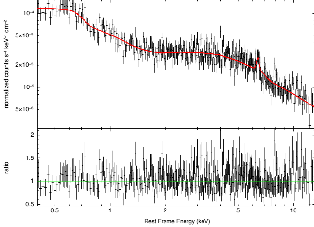
fig. 3. Comparison between the EPIC-pn spectrum and the model zxcipcf*tbabs* zpo+zga . With respect to the Fig. 1 the agreement improves especially in the band E = 0.5–1 keV, where the presence of ionization lines and edges most influences the overall shape of the spectrum. The data to model ratio is showed in the bottom panel .
