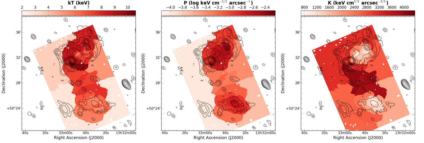
Figure 8. Thermodynamical properties of the ICM in A1758 with overlaid the LOFAR contours of Fig. 1. Images depict projected values of temperature (left), pressure (centre), and entropy (right). The temperature error map and a lower S/N temperature map are reported in Appendix A.
