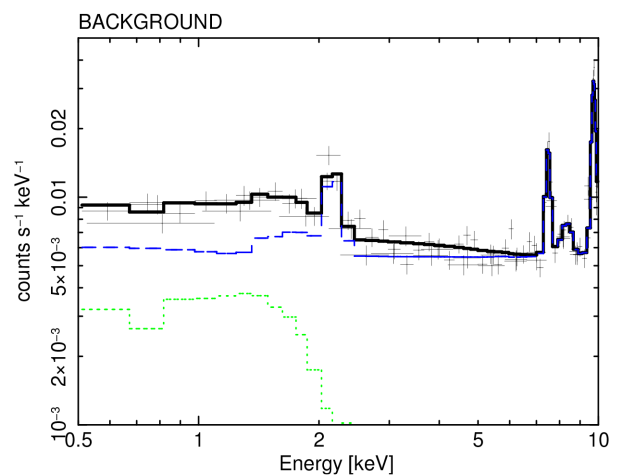
Figure 3. Spectrum of the Chandra background. Data points are shown in black together with the best-fitting model. The astrophysical and instrumental backgrounds are shown in dotted green and dashed blue, respectively. Whilst the three ObsID spectra were simultaneously fitted, the models for only one observation were reported in order to avoid confusion in the plot. The c-stat/d.o.f. of the fit is 406/386.
