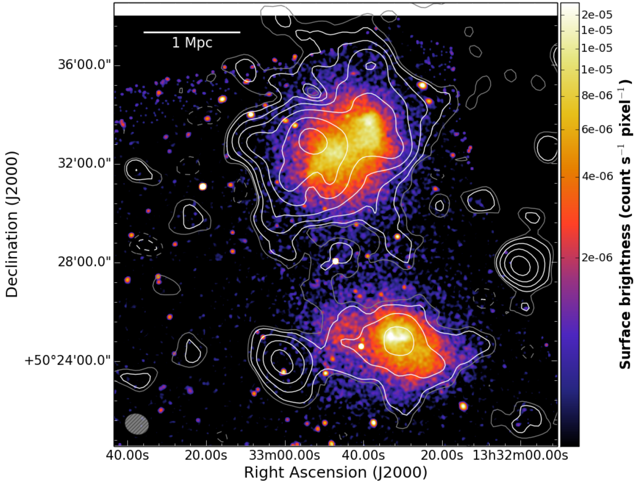
Figure 4. LOFAR radio contours with point sources subtracted of A1758 overlaid on the Chandra colour image of Fig. 2. The LOFAR white contours are spaced by a factor of 2 starting from 3\sigma , where \sigma_{\text{LOFAR}} = 390 \mu\text{Jy beam}^{-1} . The negative -3\sigma contours are shown in dashed. Grey contours correspond to the \pm 2\sigma level. The beam size is 60 \text{ arcsec} \times 51 \text{ arcsec} and is shown in the bottom left corner. More details on the LOFAR image are reported in Table 2.
