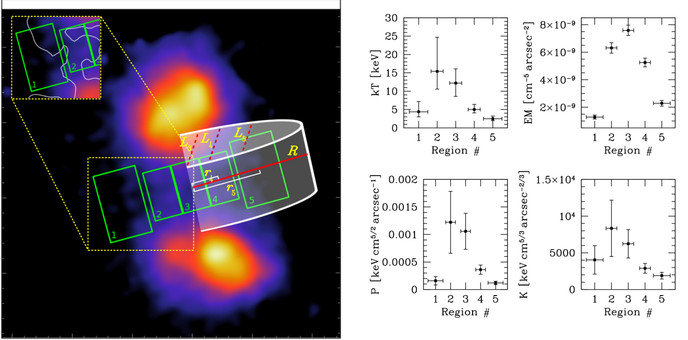
Figure 9. Left-hand panel: same Chandra image of Fig. 2 but with point sources subtracted and smoothed to a resolution of \sim 15 arcsec to highlight the X-ray channel between the clusters. The spectral extracting regions are overlaid in green. The inset panel shows the spatial coincidence between the tentative radio bridge and the putative post-shock region. The cylindrical model assumed to assess the effects of projection is also sketched. The line of sight across the i -region is L_i \sim 2\sqrt{R^2 - r_i^2} . Right-hand panels: projected values of temperature ( kT ), emission measure ( EM ), pressure ( P ), and entropy ( K ) of the X-ray channel.
