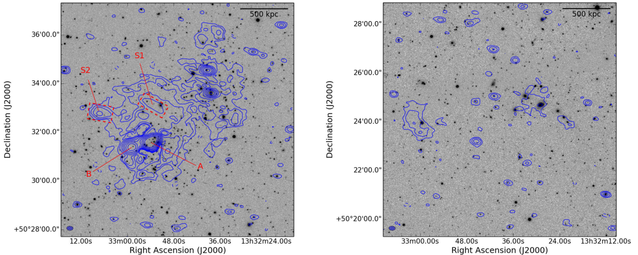
Figure 5. Mosaic SDSS g,r,i images of A1758N (left) and A1758S (right) overlaid with the LOFAR contours spaced by a factor of 2 starting from 3\sigma , where \sigma_{\text{LOFAR}} = 140 \mu\text{Jy beam}^{-1} . The negative -3\sigma contours are shown in dashed. The beam size is 16 \text{ arcsec} \times 11 \text{ arcsec} and is shown in the bottom left corners. At this resolution the radio halo in A1758S is marginally visible. More details on the LOFAR image are reported in Table 2.
