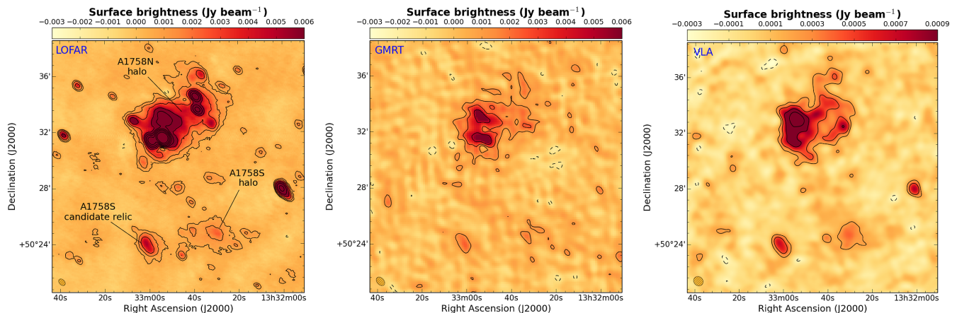
Figure 1. The cluster A1758 as observed in the radio band with LOFAR (left), GMRT (centre), and VLA (right). The point sources were subtracted in the GMRT and VLA images. Contours are spaced by a factor of 2 starting from 3\sigma , where \sigma_{\text{LOFAR}} = 230 \mu\text{Jy beam}^{-1} , \sigma_{\text{GMRT}} = 400 \mu\text{Jy beam}^{-1} , and \sigma_{\text{VLA}} = 70 \mu\text{Jy beam}^{-1} . The negative -3\sigma contours are shown in dashed. The beam sizes are 34 \text{ arcsec} \times 23 \text{ arcsec} (LOFAR), 43 \text{ arcsec} \times 29 \text{ arcsec} (GMRT), and 43 \text{ arcsec} \times 38 \text{ arcsec} (VLA) and are shown in the bottom left corners. More details on the images are reported in Table 2.
