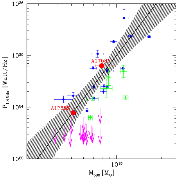
Figure 10. The P_{1.4}-M_{500} relation for giant radio haloes. Different colours indicate: giant radio haloes (blue), ultrasteepest spectrum radio haloes (green), upper limits from Venturi et al. (2008) (magenta), and the radio haloes in A1758N and A1758S (red). Errors on P_{1.4} are smaller than the point size. The best-fitting relation for giant radio haloes and its 95 per cent confidence level are shown. Adapted from Cassano et al. (2013).
