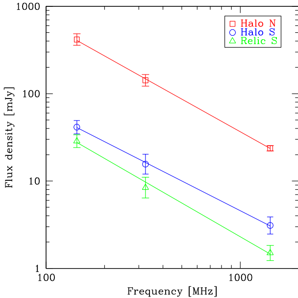
Figure 7. Integrated spectra of the diffuse radio emissions in A1758. The spectral index values are reported in Table 3.
