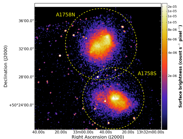
Figure 2. Chandra exposure-corrected image in the 0.5–2.0 keV band of A1758 smoothed to a resolution of \sim 3 \text{ arcsec} . Yellow circles indicate the approximate location of r_{500} for each cluster.
