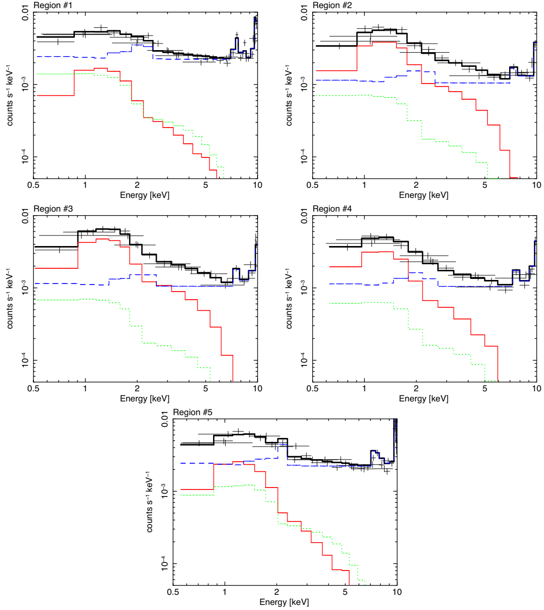
Figure B1. Spectral fitting results for the five regions shown in Fig. 9 (left-hand panel). Data points are shown in black together with the best-fitting model. Different colours denote the components of the spectral model; i.e. the cluster emission (in solid red), the astrophysical background (in dotted green) and the instrumental background (in dashed blue). Whilst the three ObsID spectra were simultaneously fitted, the models for only one observation were reported in order to avoid confusion in the plot. The c-stat/d.o.f. of the fits from region 1 to 5 are: 232/184, 135/127, 114/132, 115/113, and 224/182.
