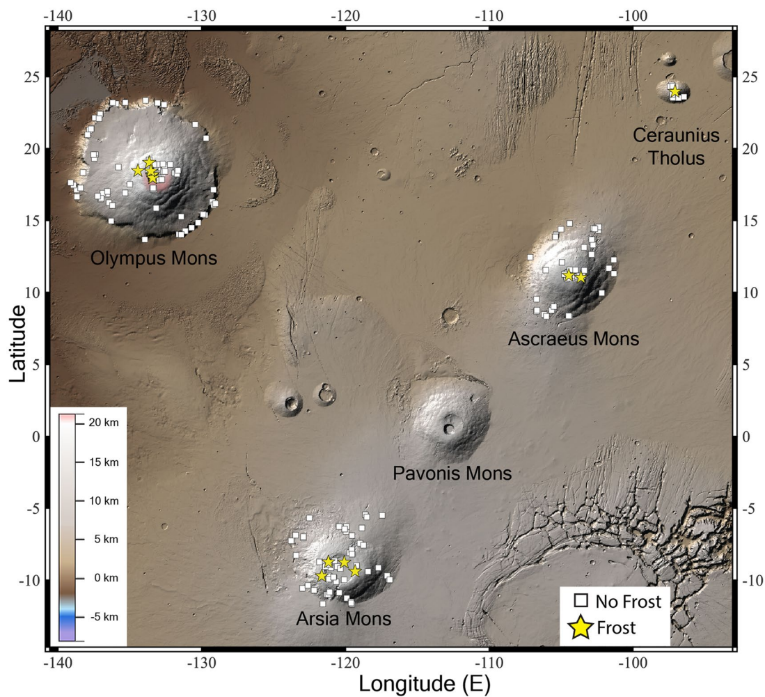
Extended Data Fig. 3 | CaSSIS frost detections in the Tharsis volcanic region. Frost was detected only on and around the calderas of the three largest volcanoes such as Olympus, Arsia and Ascraeus Montes, but also on the smaller Ceraunius
