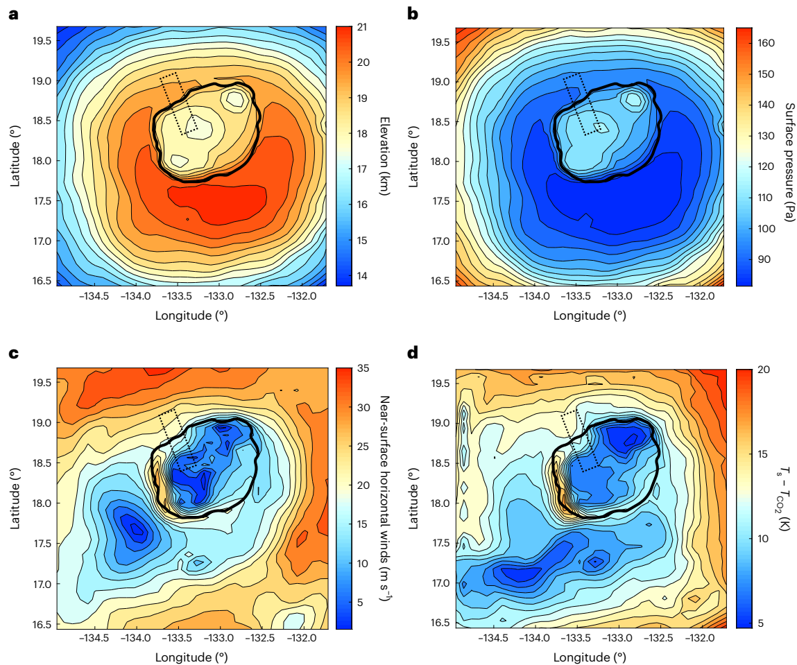
Fig. 5 | Microclimatic conditions simulated over Olympus Mons. a–d , Utilizing MarsWRF high-resolution mesoscale modelling (at the time of CaSSIS observation Fig. 1d), this figure presents the influence of Olympus Mons’s topography on its local climate, as shown by elevation gradients ( a ), surface atmospheric pressure ( b ), near-surface horizontal wind patterns ( c ) and the deviation in temperature between the Martian surface and the local CO 2 frost point ( d ). The topography of the Olympus Mons caldera is demonstrated to
