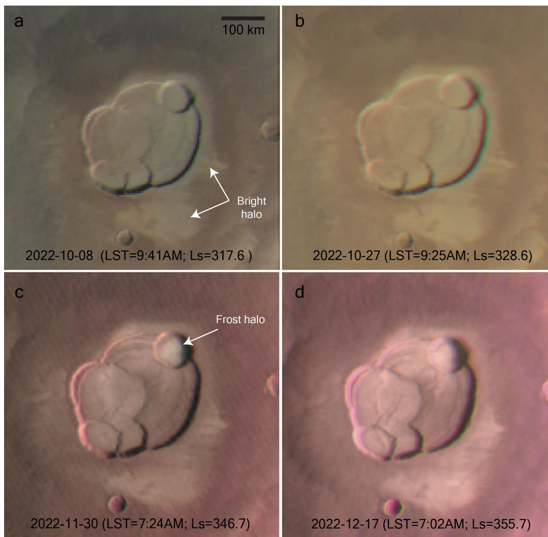
Extended Data Fig. 1 | Diurnal variations of frost halo on Olympus Mons. HRSC images of Olympus Mons (lat = 18.2°N, lon = -133.2°E) acquired at different local times in MY 36. (a, b) Late morning images showing no evidence of frost on the bright halo deposit surrounding the volcano caldera. (c, d) Early morning images revealing the presence of frost on the bright halo deposit. The bright halo
