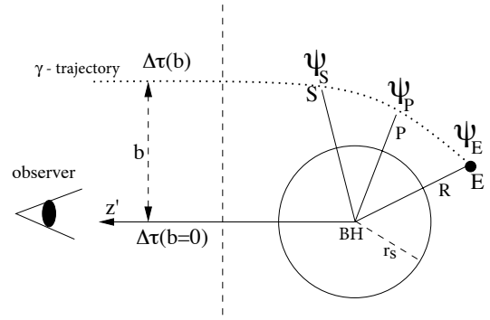
Fig. 2. Calculation of travel time delay for trajectories with turning points. The photon is emitted at E with radius R and deflection angle \psi_E . The photon trajectory passes through point S , which is symmetric to E with respect to periastron p , having the same impact parameter, b , and a deflection angle \psi_S = 2\psi_p - \psi_E .
