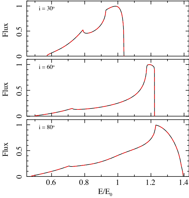
Fig. 8. Line profile for isotropic radiation from R_{\text{in}} = 3 r_s to R_{\text{out}} = 50 r_s assuming surface emissivity q = -3 . The continuous black lines represent the original equations and the dashed red lines are the polynomial approximate equations.
