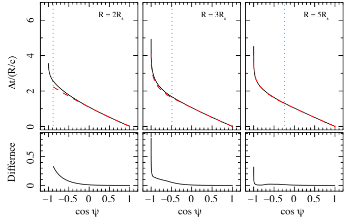
Fig. 4. Continuous black curves are obtained from the original time delay Eq. (5), while the dashed red curves are from the polynomial approximate Eq. (22). Different panels show R = 2r_s , R = 3r_s and R = 5r_s . The dotted blue line helps distinguishing trajectories without a turning point (i.e., 0 \leq \alpha \leq 1 ) from those with a turning point (i.e., \pi/2 \leq \alpha \leq \alpha_{\max} ). The lower panels show the difference between the curves from the original and approximate equations.
