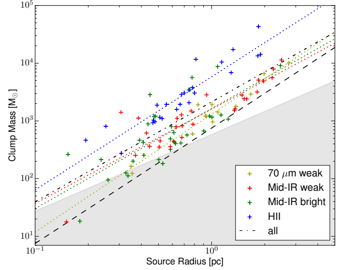
Fig. 10. Mass-size relationship of the ATLASGAL Top100. The lower right grey shaded area highlights the region where it is unlikely that high-mass stars are formed according to Kauffmann et al. (2010) and the black dashed line indicates a surface density of 0.05 \text{ g cm}^{-2} determined as the lower limit for efficient massive star formation by Urquhart et al. (2014c). Note that the slopes of the linear log-log fits of all classes agree with each other within the margin of error of the fitted power laws.
