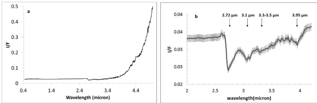
Fig. 1 Average Ceres' spectrum. a) Average spectrum of Ceres from 0.4 to 5 \mu\text{m} . No smoothing has been applied to the spectrum and some instrument artifacts are still present, especially in the thermal range (4.2-4.6 \mu\text{m} ). The error bars are calculated taking into account a mean absolute deviation of the calibration uncertainties along the 256 samples. Errors bars are not shown for clarity, but are of the same order of those in b. b) Expanded thermal-removed average Ceres spectrum in the 2-4.2 \mu\text{m} range.
