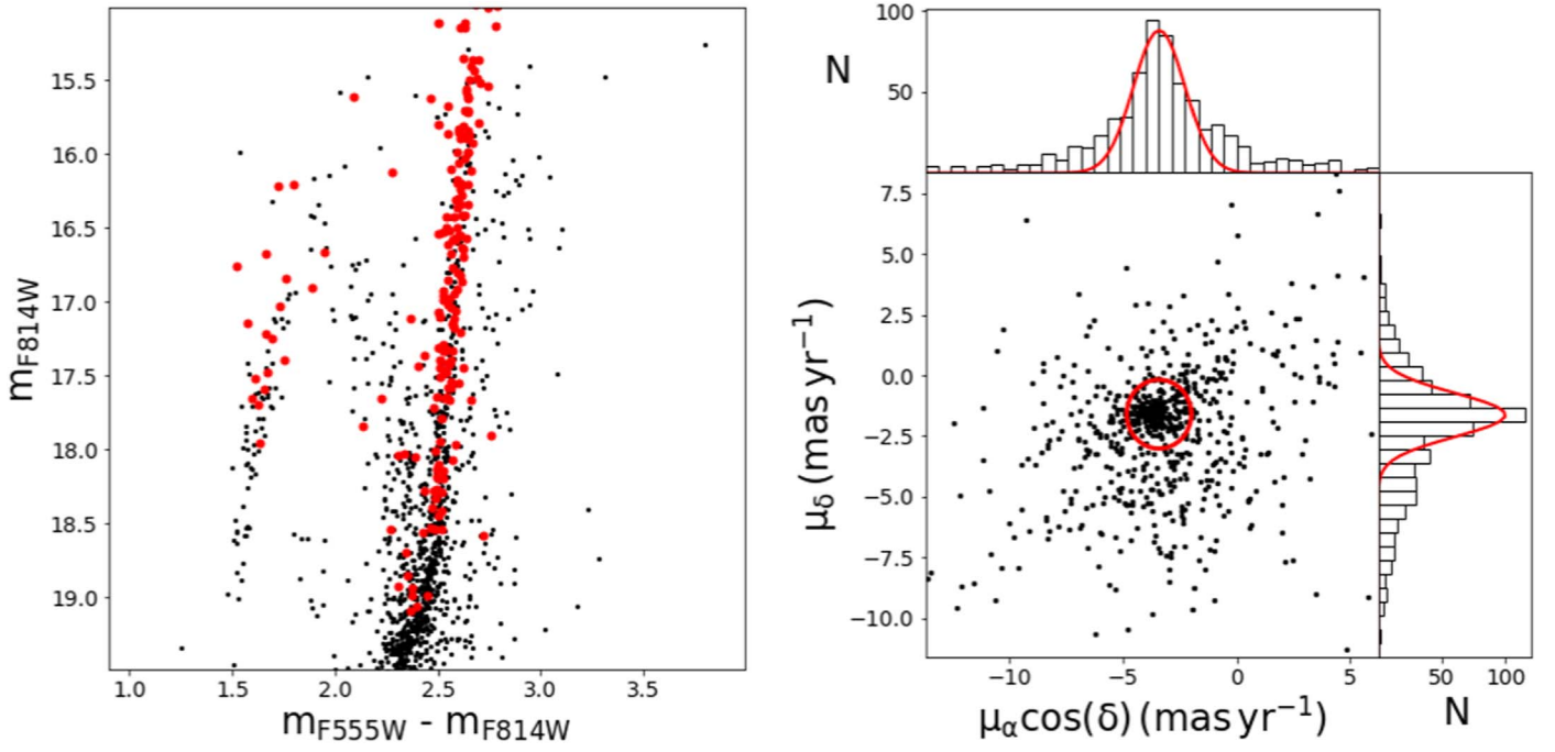
Figure 8. Left panel: differential reddening-corrected CMD of NGC 6256 (same as in the right panel of Figure 1), showing only the stars in common with the Gaia DR2 catalog. The red dots correspond to the stars included within the red circle shown in the VPD in the right panel of the figure. Right panel: the main panel shows the VPD of the stars in common between our HST catalog and the Gaia DR2 catalog. The upper and side plots show the histograms of the PMs along R.A. and decl., with a best-fit Gaussian function superimposed. The red circle in the main panel is centered on the mean values of the best-fit Gaussian functions and has a radius of 1.4 \text{ mas yr}^{-1} , equal to the combined 1\sigma values. This circle encloses all the stars that have been used to measure the cluster absolute PM.
