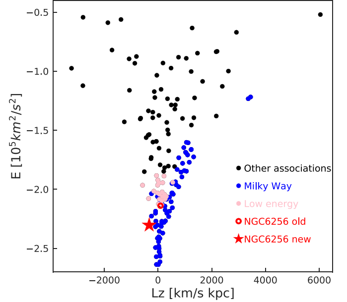
Figure 10. Integrals of motion for the sample of Galactic GCs analyzed in Massari et al. (2019). Blue points are clusters belonging to the Galaxy in situ population, pink points are those associated with an accreted low-energy component while black points are clusters with different associations. The position of NGC 6256 previously computed by Massari et al. (2019) is reported with a red open circle while its updated position is shown with a red star.
