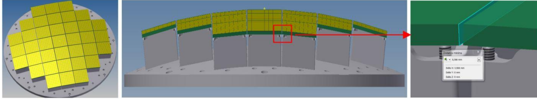
Figure 1. ASTRI camera focal plane assembly. The telescope curved focal plane imposes the arrangement of detection modules and the maximum allowable dimensions of the tiles.
