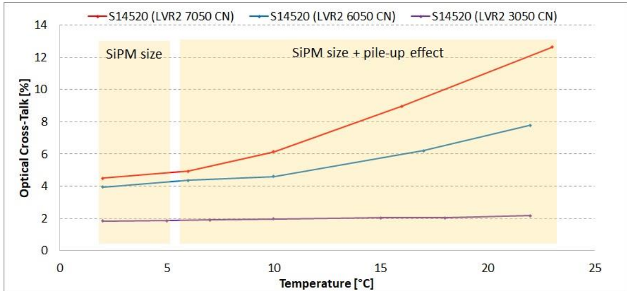
Figure 8. OCT versus temperature. Below 5°C, the OCT depends only by the SiPM size while above 5°C the OCT is affected by the pile-up effect, or better to say the electronic front-end operates an inadequate PZC.
