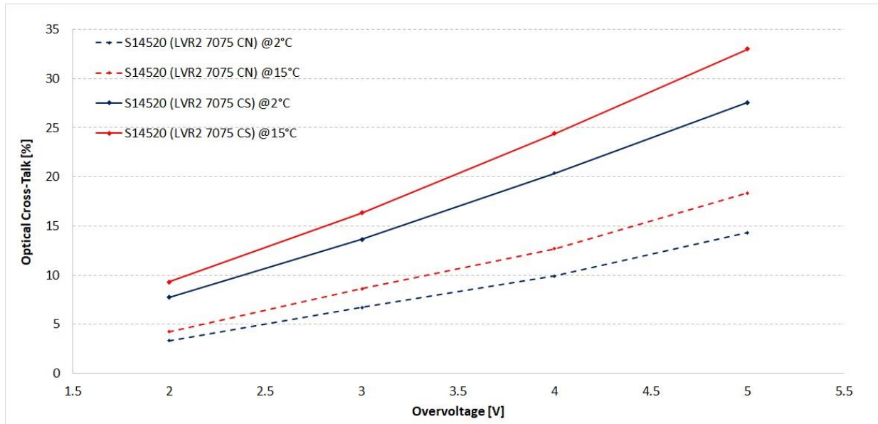
Figure 9. OCT versus overvoltage at 2°C and at 15°C. The CN series shows a lower OCT respect to the CS series because the protective coating in the CS series. The electronics is responsible for the different behaviour at the two temperatures.
