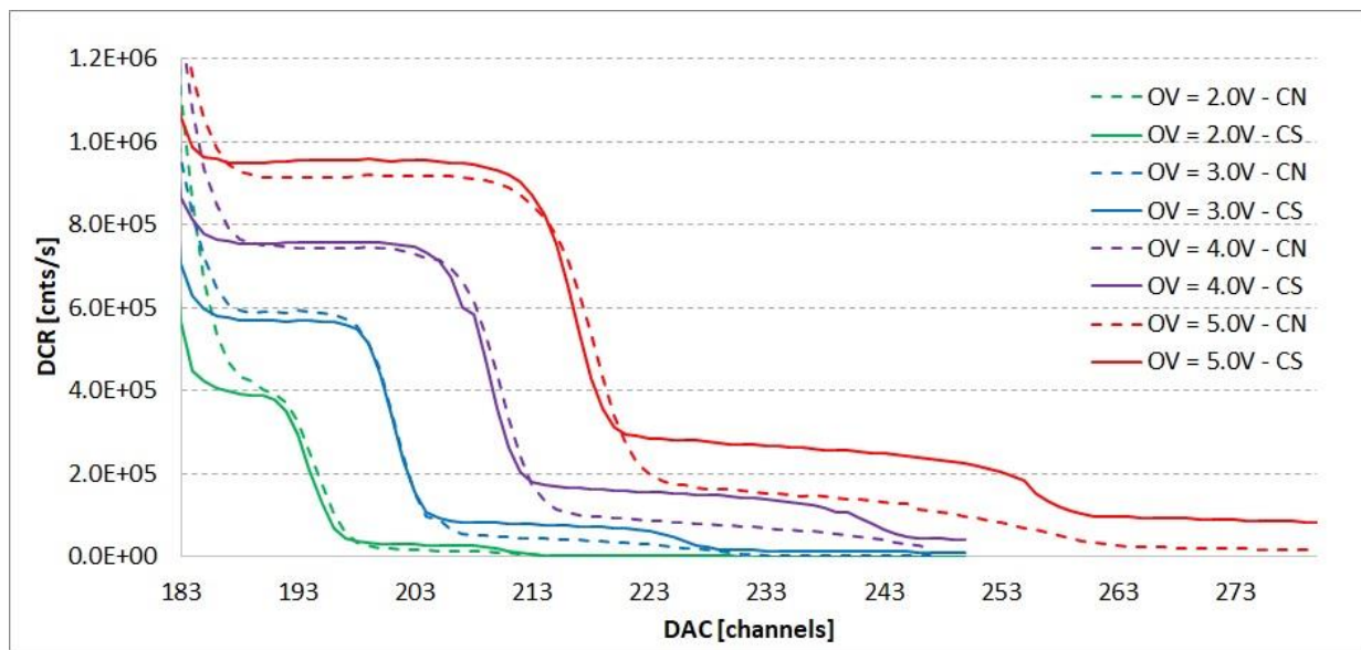
Figure 7. DCR curves for the characterized S14520 (LVR2 7075 CS) and S14520 (LVR2 7075 CN) detectors as a function of the discriminator threshold at 3°C operating temperature. The difference in the second p.e. is clearly evident and implies a reduced OCT in the CN series device.
