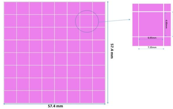
Figure 2. 8 \times 8 -pixels tile schematics. Using 7 \times 7 \text{ mm}^2 SiPMs 57.4 \times 57.4 \text{ mm}^2 can be assembled. On the right part a detail of a single 7 \times 7 \text{ mm}^2 pixel is shown. With this configuration a total area of 3294.75 \text{ mm}^2 , an active area of 3091.36 \text{ mm}^2 and a filling factor of 93.83% are achieved.
