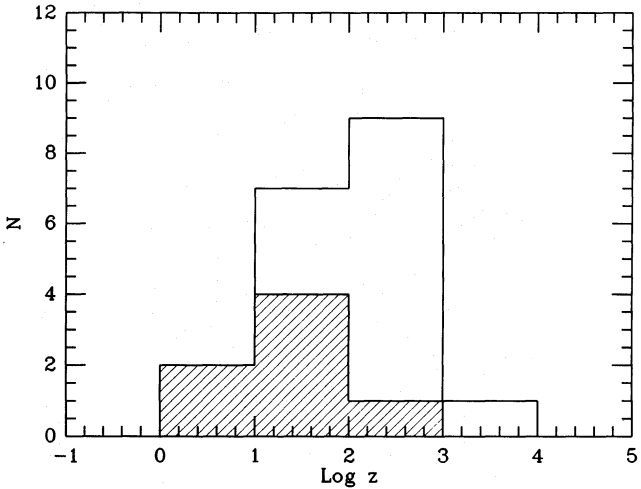
Fig. 5. Histogram showing the frequency distribution as a function of \log(z) for slow novae from the “fiducial sample” (unshaded area) and fast novae of the “fiducial sample” (the shadowed area)
