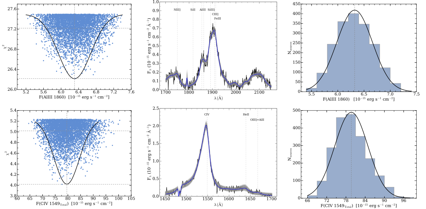
Fig. B.1. Left panels: distribution of \chi^2 as a function of the flux of AlIII (top) and total CIV profile (bottom). Black continuous lines mark the normal distribution associated with simulations. Gray horizontal lines indicate the value at \chi^2_{\min} and at \chi^2_{\min} + 1 . The gray vertical line indicates the mean of the normal distribution. Middle panels: spectra of the quasar SDSSJ222753.07-092951.7 in the 1900 Å blend (top) and total CIV 1549 (bottom) spectral ranges. Gray shadow regions correspond to the models at the \chi^2_{\min} + 1 confidence level obtained from the Monte Carlo simulations. The blue line corresponds to the SPECFIT result. Right panels show the distributions of the fluxes of AlIII (top) and total CIV (bottom) for all the models under the 1σ confidence level plotted in the left panels. Vertical lines has the same meaning as in left panels.
