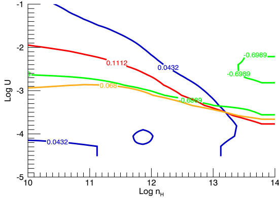
Fig. 7. Isocontours in the plane log of ionization parameter ( U ) versus log of hydrogen density ( n_H ) from CLOUDY simulations for the line intensity ratios \text{AlIII}\lambda 1860/\text{SiIII}\lambda 1892 (blue), \text{HeII}\lambda 1640/\text{CIV}\lambda 1549 (green), \text{CIV}\lambda 1549/\text{AlIII}\lambda 1860 (yellow), \text{CIV}\lambda 1549/\text{SiIII}\lambda 1892 (red) using Z = 100 Z_\odot . Labels report the median values of the intensity ratios for the objects of the GTC-xA sample.
