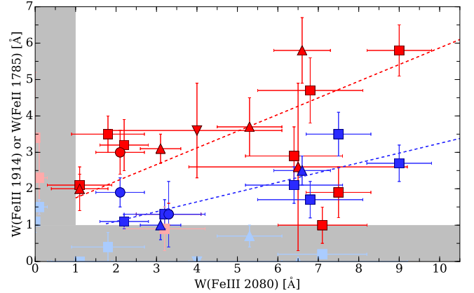
Fig. 8. Relation between intensity of the FeIII feature at 2080 Å with Fe UV 1785 Å (blue) and FeIIIλ1914 (red). Squares, up and down triangles, and circles mark the normal, BAL, mini-BAL and RL quasars, respectively. The gray shaded area indicates an approximate detection limit. Blue and red lines mark the orthogonal fit for each case.
