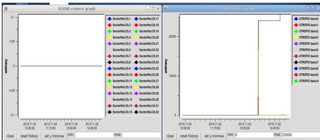
Fig. 15: ELINA & STROFIO Science 2015-11-02
