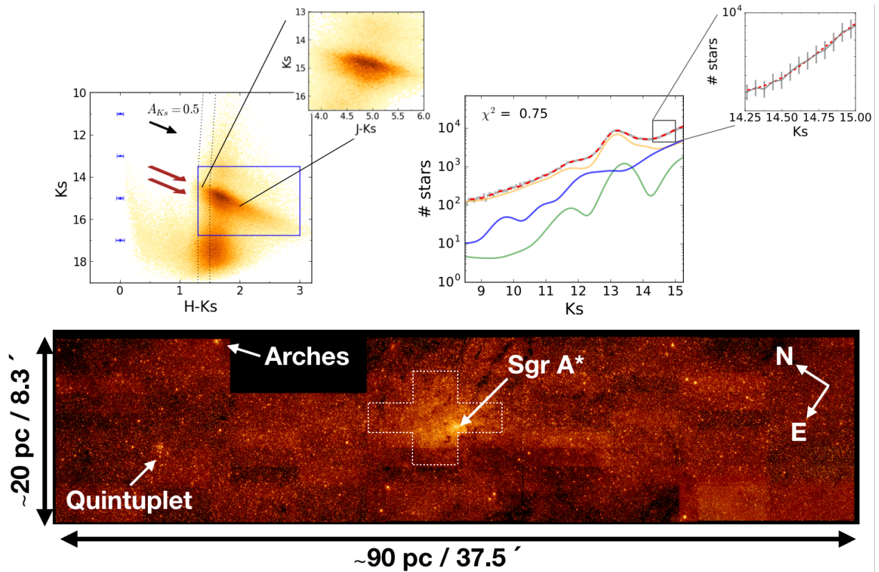
Fig. 1: Lower panel: Ks-band image of the GALACTICNUCLEUS survey region examined for this study. The positions of Sgr A*, the Arches and the Quintuplet clusters are indicated. The cross-shaped region outlined by a white dashed line was excluded because of too high source crowding. The dark rectangle right next to the Arches cluster is a field with incomplete data. Upper left: Observed H-Ks CMD. The vertical dashed lines show the two colour cuts used to exclude foreground stars (see Methods). The two arrows indicate the direction of reddening and point toward the two parallel features that we detected in the RC, corresponding to old (brighter) and younger (fainter) stars. The inset shows the double RC in the J-Ks CMD. The blue rectangle indicates the stars used to create the extinction map. The error bars, in blue, show the uncertainties for different magnitude bins. Upper right: KLF (grey), obtained after extinction correction of the observed stars, and best-fit model of the star formation history (red dashed line). For simplicity we combined the theoretical LFs used into old, intermediate and young ages (orange, green and blue, respectively). The zoom shows the quality of the data in detail, including error bars and model fit.
