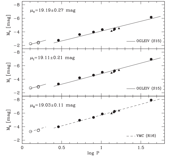
Figure 10. Predicted PL relation in the V (top panel), I (middle panel) and K (bottom panel) bands based on the model fitting results for both F (black solid circles) and FO Cepheids (open circles). The empirical relations by the OGLE IV (solid lines) and VMC (dashed line) collaborations are shown for comparison and used in combination to the predicted absolute magnitudes to infer the labelled distance moduli.
