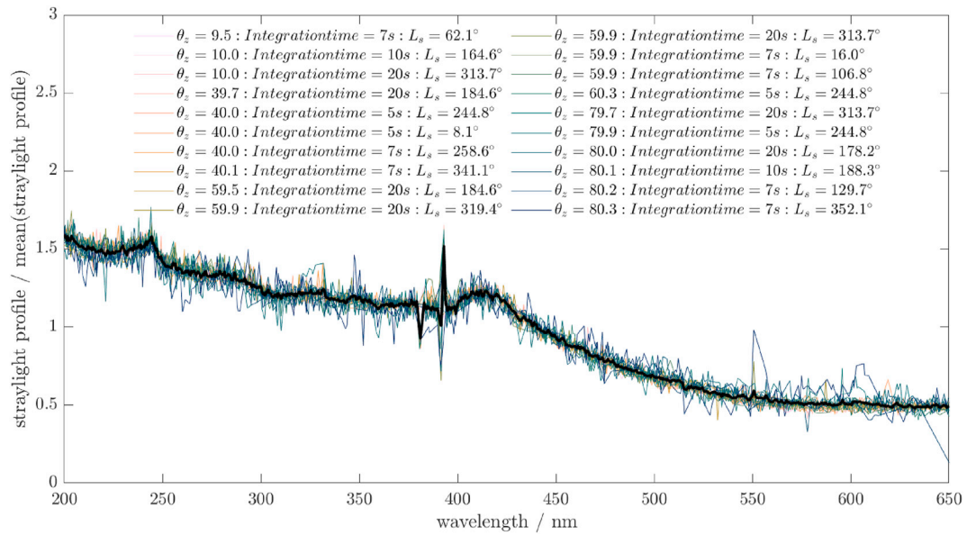
Fig. 5. The inflight straylight profile as a function of wavelength at pixel position ( p_{m,io} - p_{s,io} ) in the NLR for different, solar zenith angles, location, integration times and time of year. Each straylight profile has been normalised to the mean of itself across all wavelengths to emphasise that the straylight is independent of the incident flux, integration time and has been stable over the course of the UVIS science mission. The mean straylight structure as a function wavelength is shown by the black line.
