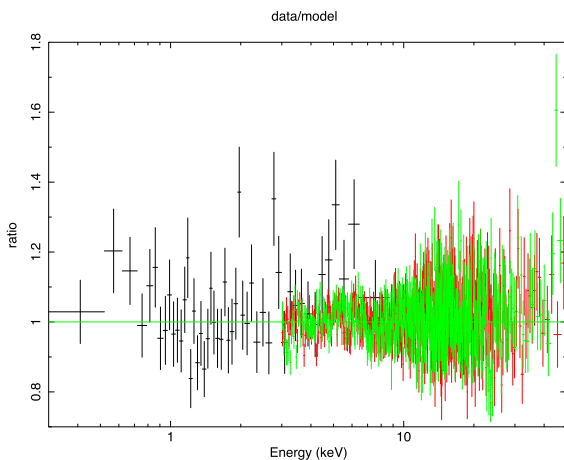
Figure 7 Data-to-model ratio for the summed observations of 4C 74.26, employing the relxillfp model, following Lohfink et al. (2017).
