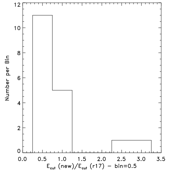
Figure 6 Left-hand panel : plot of the values of the high energy cut-off from the present analysis plotted against the results from Ricci et al. (2014) (cyan circles) and from several studies employing solely NuSTAR data (red triangles); the 1:1 line is shown for reference. Right-hand panel : histogram of the ratio between the high energy cut-off values measured in this work and those obtained by Ricci et al. (2014).
