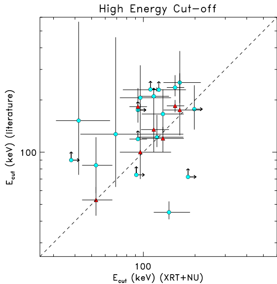
Figure 6 Left-hand panel : plot of the values of the high energy cut-off from the present analysis plotted against the results from Ricci et al. (2014) (cyan circles) and from several studies employing solely NuSTAR data (red triangles); the 1:1 line is shown for reference. Right-hand panel : histogram of the ratio between the high energy cut-off values measured in this work and those obtained by Ricci et al. (2014).
