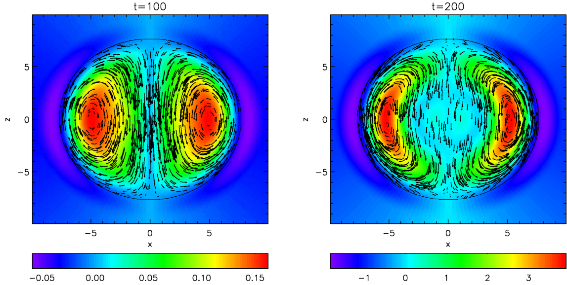
Figure 1. DC-GRMHD magnetar model. The magnetic field configuration at two different times of evolution, t = 100 and t = 200 . Fieldlines refer to the poloidal component, whereas color contours to the toroidal one, with values expressed in units of 10^{15} G.
