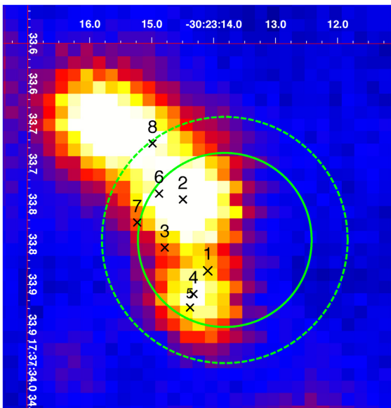
Figure 6. UKIDSS infrared map ( K band) of the sky region around IGR J17375–3022, superimposed on the Swift/XRT error circles at 90 per cent and 99 per cent confidence level. Sources numbered from 1 to 8 are listed in Table 2.
