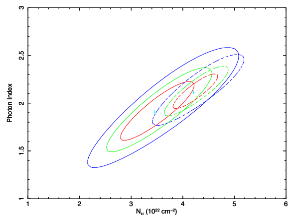
Figure 5. Confidence contour levels (68 per cent, 90 per cent, and 99 per cent) for the two parameters of the absorbed power-law model applied during the spectroscopy of IGR J17375–3022 Swift / XRT observations ID 31278001 (solid lines) and 31278002 (dashed lines).
