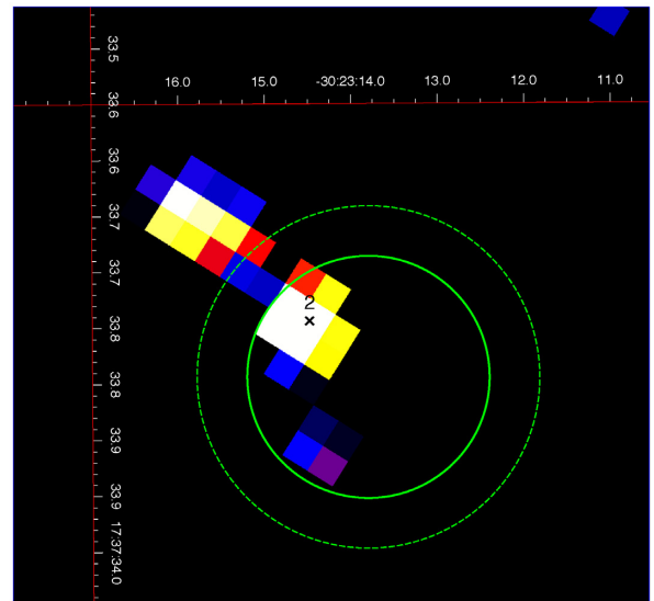
Figure 7. VVV infrared map ( K band) of the sky region around IGR J17375–3022, superimposed on the Swift/XRT error circles at 90 per cent and 99 per cent confidence level.
