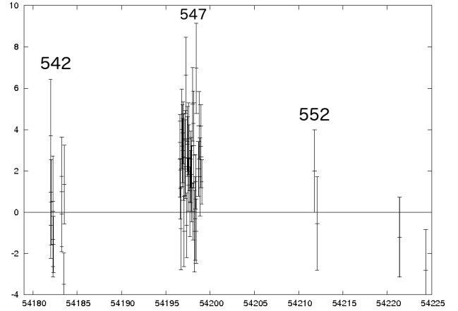
Figure 10. IBIS/ISGRI light curve (18–60 keV) at ScW level of XTE J1829–098 covering the period from revolution 542 to 552.
