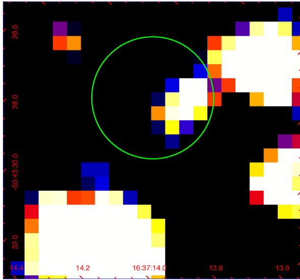
Figure 3. Spitzer infrared map from the GLIMPSE survey (3.6 \mu\text{m} band) of the sky region around IGR J16374–5043, superimposed on the Swift / XRT error circle at 90 per cent confidence level.
