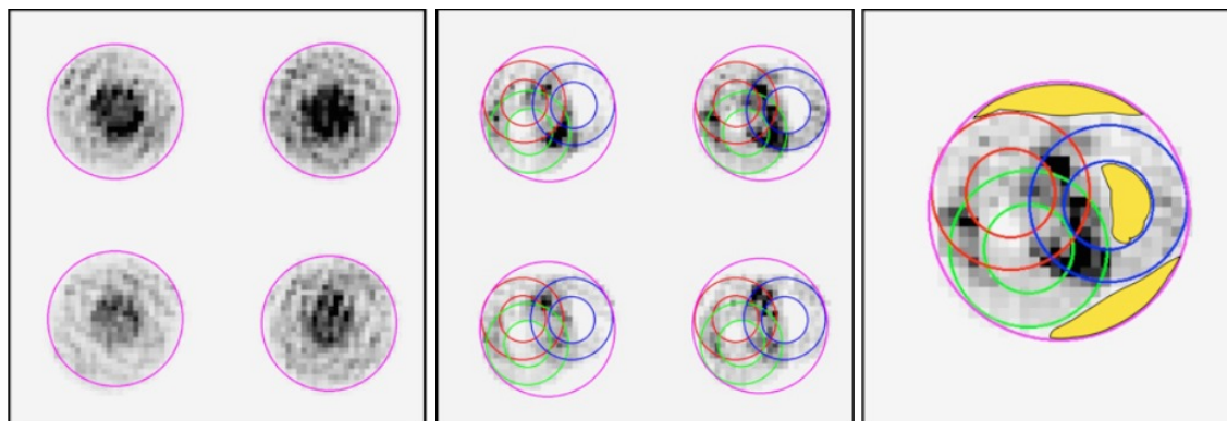
Figure 2. Real images from the HWS. The purple circle represents the meta-pupil projection on to the CCD. left : fully-illuminated image; middle : partially-illuminated metapupil image; right : one of the quadrants of the middle panel. The yellow shaded regions are the non-illuminated sub-apertures.
