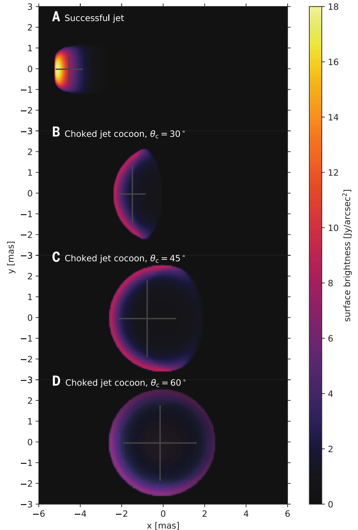
Fig. 2. Predicted source images for our four models. (A) Predicted radio brightness distribution at 207.4 days for the structured jet model. (B to D) Same as (A), but for the choked jet cocoon model with effective opening angles of \theta_c = 30^\circ (B), 45^\circ (C), and 60^\circ (D). Gray crosses show the positions and sizes (full widths at half maxima) of elliptical Gaussian fitting of the images. The coordinate origin, in each image, is the projected position of the binary neutron star merger (16).
