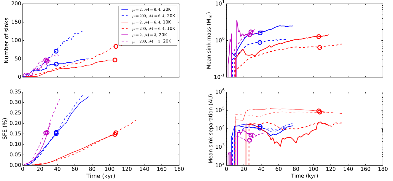
Fig. 7. Left: Time evolution of the number of sink particles (top) and of the SFE (bottom) for simulations (2), (3), and (4), i.e. the simulations that reproduce the collapse of a 300 M_{\odot} clump. The circles indicate the time at which we postprocessed the simulations, which corresponds to a \text{SFE} \approx 15\% . Right: Time evolution of the mean sink particle mass (top) and of the mean separation between sink particles (bottom). The thin lines show the mean separation calculated by accounting for the sink particles located within a sphere of radius 40 000 au around the most massive one. The dashed lines show the mean separation between all the sink particles.
