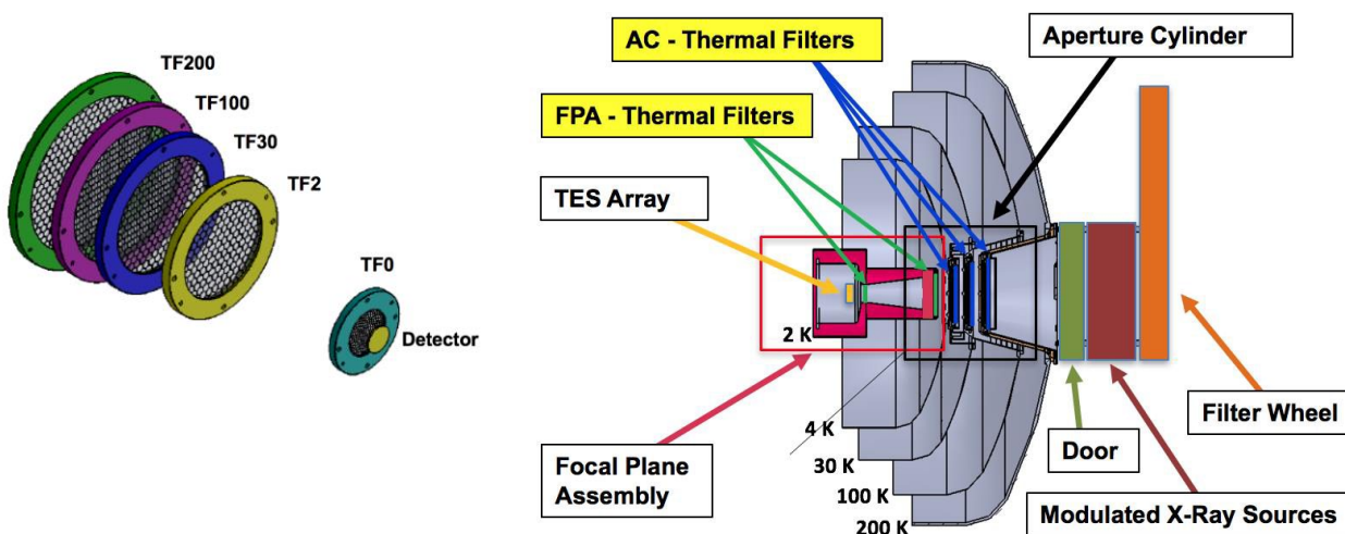
Figure 1. Schematic view of the five thermal filters with distances from the detector and diameter in proper scale (left panel). The right panel shows the thermal filters inside a schematic drawing of the DCS together with the major instrument subsystems.
