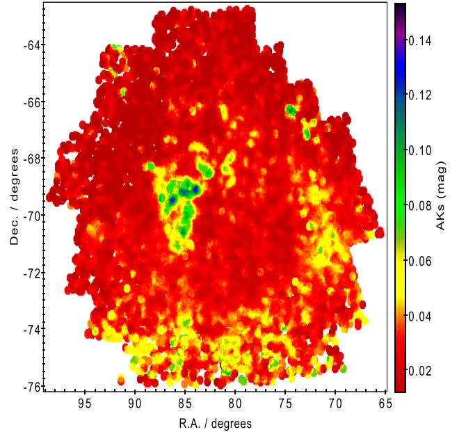
Figure 4. K_s -band absorption map derived from the RRL stars. The position of each RRL was re-binned to a circle of 30 arcsec in diameter.
