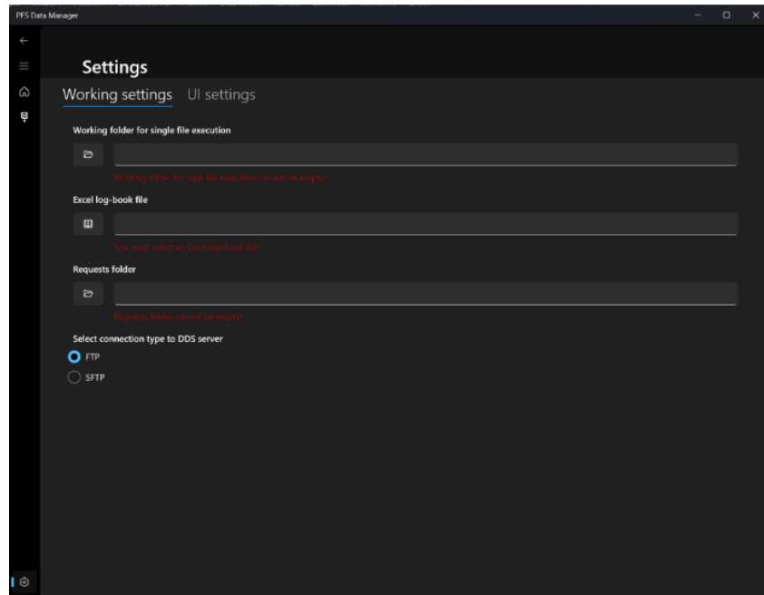
Figure 5 Settings page
