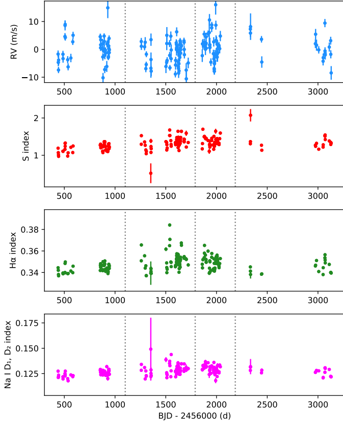
Fig. 1. From top to bottom: original RV (derived with the TERRA pipeline), S-index, H \alpha -index, and Na I D 1 , D 2 -index time series for GJ 9689. Vertical dotted lines indicate the first three observing seasons as used in our study.
