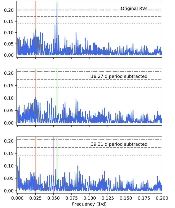
Fig. B.1. Top: GLS periodogram of the DRS RV measurements. Middle: GLS periodogram after subtracting the 18.27 d period. Bottom: GLS periodogram after subtracting the 18.27 and the 39.31 d signals. Values corresponding to a FAP of 10, 1, and 0.1% are shown with horizontal grey lines. The vertical red line indicates the period at 39.31 d, while the vertical green line shows the 18.27 d period. The first harmonic of the 39.31 d signal is shown in violet.
