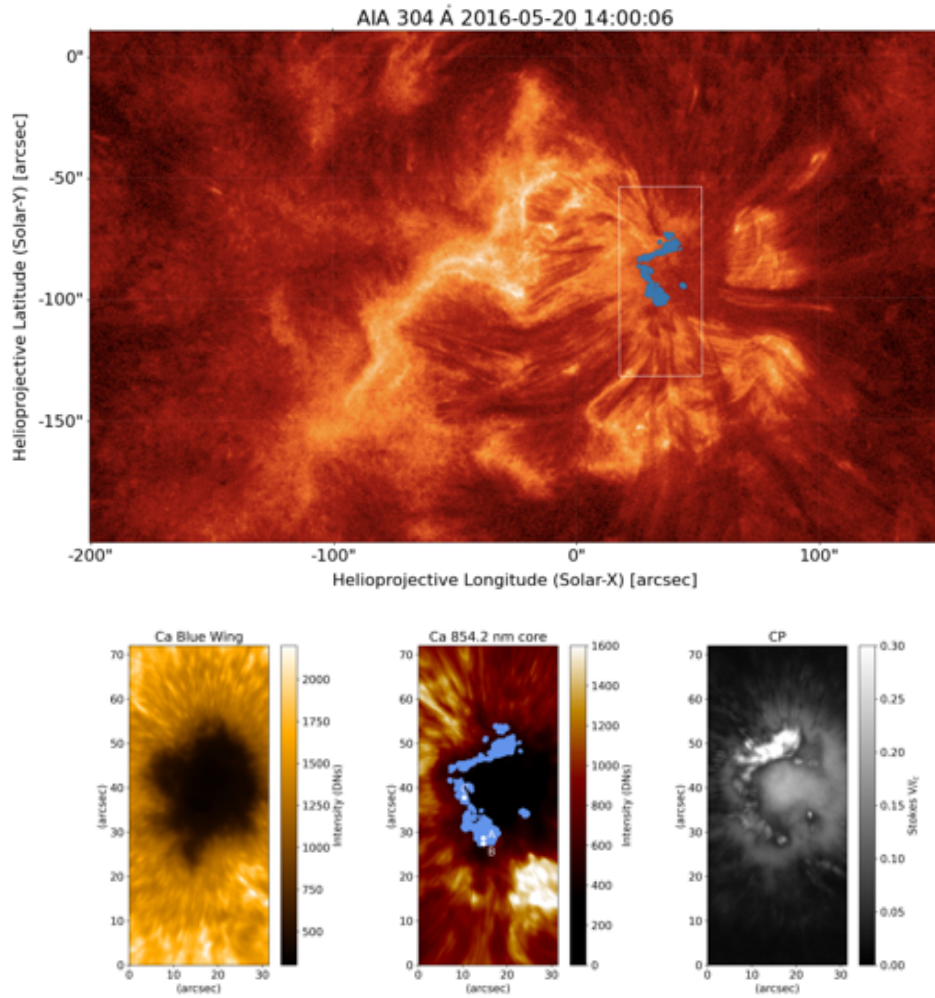
Figure 1. Upper panel: SDO/AIA He II 304 nm context image of AR 12546. Bottom left: IBIS narrow band intensity image in the blue wing of the Ca II 854.2 nm spectral line. Bottom center: IBIS intensity image in the core of the Ca II 854.2 nm spectral line. The blue dots indicate the positions where there exists a large ( > 95\% ) coherence between the intensity and CP fluctuations (see text). The three white dots indicate the positions corresponding to the wavelet diagrams shown in Fig. 2. Bottom right: Ca II 854.2 nm circular polarisation map.
