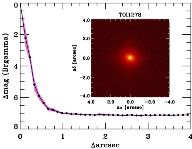
Figure 2. Br \gamma 5 \sigma contrast curve of TOI-1278 from Palomar/PHARO NIR adaptive optics imaging. No close companion is detected.
