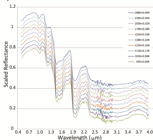
Fig.1- Scaled spectra of Hexahydrite 20–50 \mu\text{m} at different T. Spectra are offset for clarity.
