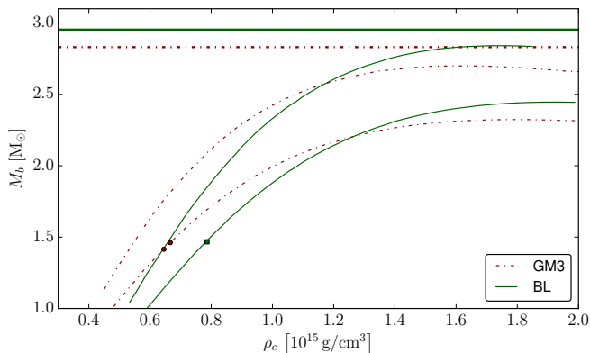
FIG. 1. Baryonic mass as a function of central rest mass density of non-rotating (lower curves) and maximally uniformly rotating (upper curves) NSs for the two EOSs used in this paper (BL and GM3). The horizontal lines represent the masses of the BNS systems, while the markers on the curves represent the mass values for the single NSs in the binary.
