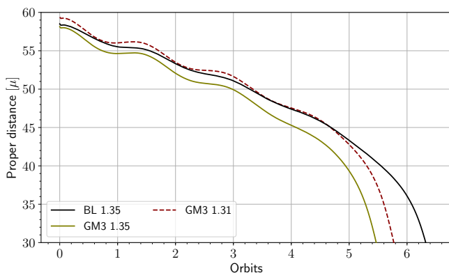
FIG. 3. Proper separation between the NS barycenters during the inspiral as function of orbital phase. The separation is given in units of reduced mass \mu = M_g^1 M_g^2 / (M_g^1 + M_g^2) . The barycenters and orbital phases are computed using simulation coordinates.
