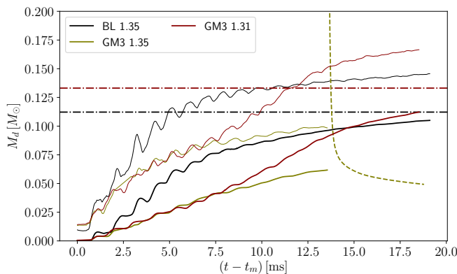
FIG. 7. Time evolution of disk mass for our simulations. The solid thick lines show the disk mass measure M_d , and the thin solid lines the alternative measure M_d^{\text{alt}} . After the BH formation for model GM3-1.35 , we show the mass outside the apparent horizon instead (dashed line). The rapid initial decrease corresponds to the rapid initial growth of the apparent horizon. The horizontal lines mark a disk mass for which the remaining remnant mass is at the upper limit for a SMNS (the two GM3 models are indistinguishable due to almost identical total mass).
