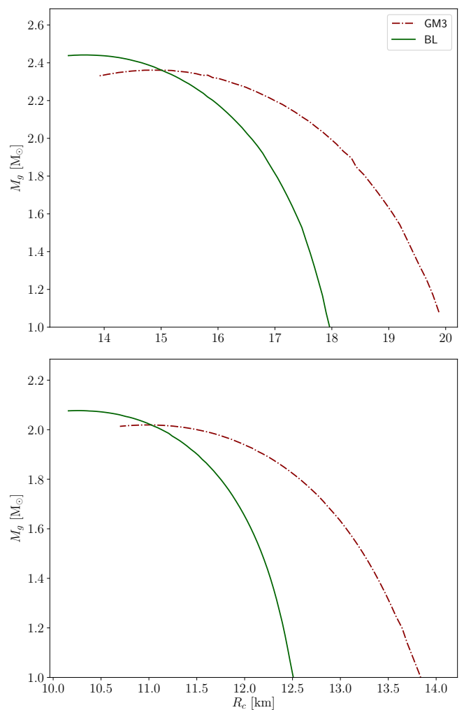
FIG. 2. Gravitational mass as a function of circumferential radius of NSs depending on the chosen EOS. Bottom panel: relation for non-rotating NSs. Top panel: relation for NSs rotating uniformly at mass shedding limit.
