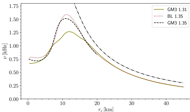
FIG. 8. Rotation profile of the remnant for our models 11 ms after merger. r_c is the circumferential radius, and \nu the rotation frequency as observed from infinity. The dash-dotted curve represents the frequency for a test particle on a prograde circular orbit.
