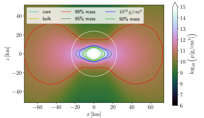
FIG. 6. Structure of the disk and embedded remnant for model GM3 - 1.31 , at the end of the simulation. The mass density is shown as color plot. In order to remove contributions from oscillations, we average in time over the last 4 ms. The white circle marks the cutoff (coordinate) radius used to define the disk mass M_d . The density cutoff 10^{13} \text{ g/cm}^3 used for the alternative definition M_d^{\text{alt}} is marked by the blue contour. The other contours mark isodensity surfaces containing 90, 95, and 98% of the total baryonic mass, and those corresponding to remnant bulk and core (see text).
