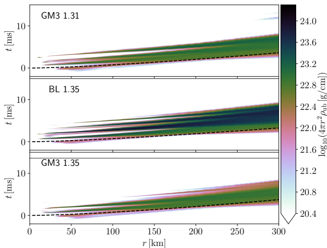
FIG. 11. Radial distribution of unbound matter as a function of time. The logarithmic color scale corresponds to the unbound mass per coordinate radius. The black dashed line represents the trajectory of a radially outgoing test mass with velocity v_\infty from Table III. The trajectory has been estimated using the Newtonian potential of a mass equal to the ADM mass at the end of the simulation.
