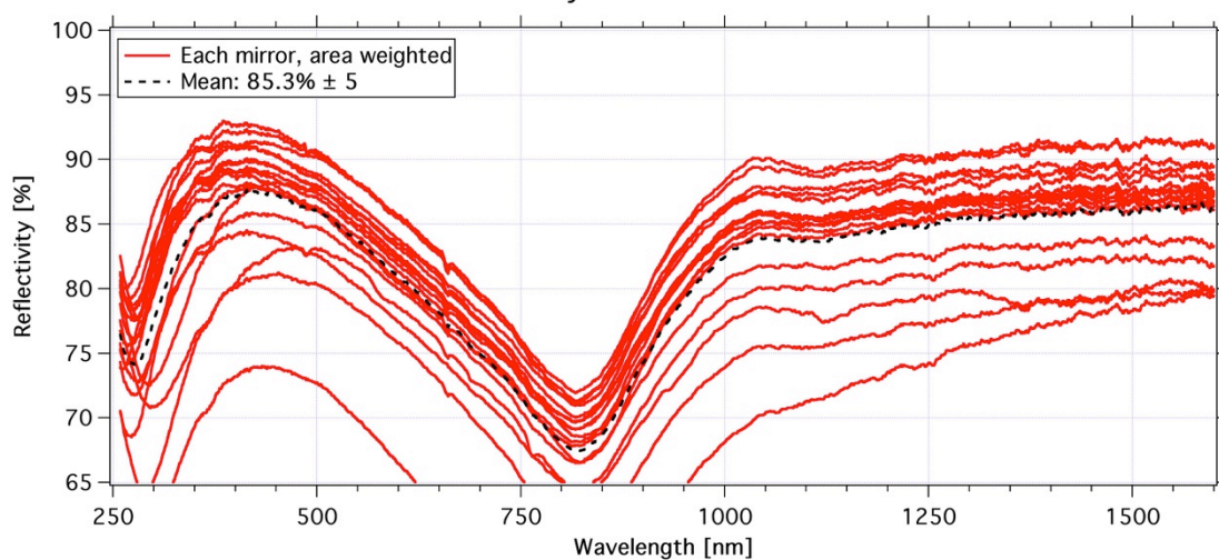
ASTRI-SST-2M Reflectivity of M1 - Data taken on 20151120
