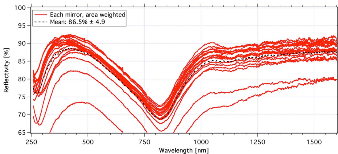
ASTRI-SST-2M Reflectivity of M1 - Data taken on 20150330
