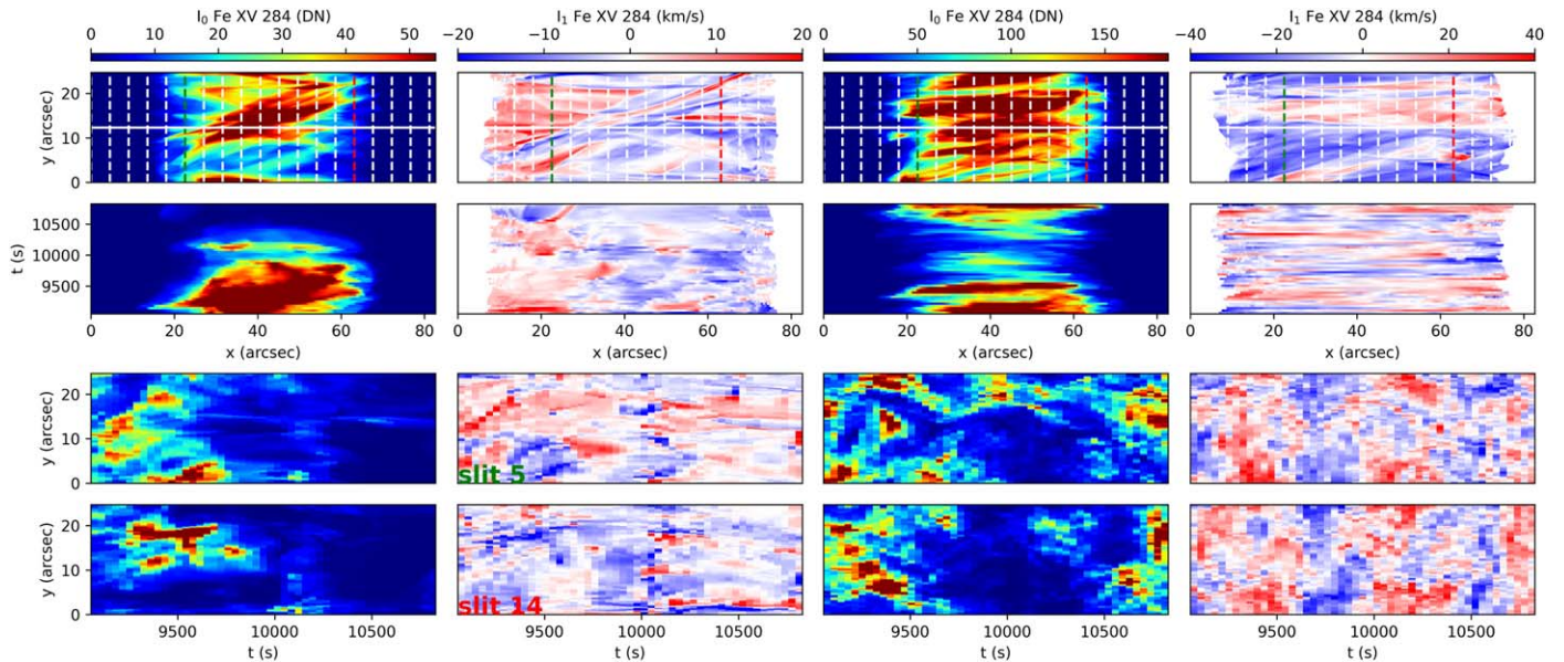
Figure 12. Comparisons between MUSE observables predicted by idealized numerical loop models in which loop footpoints are shuffled by either driver on DC-like (model La_DC ; see Section 2 and Appendix A) or AC-like (model La_AC ) timescales (see Howson et al. 2020 for a detailed explanation of the driving timescales)—i.e., mimicking heating by braiding or waves, respectively—show clear differences. We show the intensity and Doppler velocity for the DC (left two columns) and AC (right two columns) model in the MUSE Fe XV 284 Å line integrated over 1.5 s. The top row shows a snapshot at t = 9054 s where x represents the field-aligned coordinate. The LOS has been taken to be perpendicular to the magnetic field. The second row shows a time–distance image along the central y coordinate (horizontal white line in the top row). The third and fourth rows show time–distance images in the cross-field direction along slit 5 (vertical dashed green line in the top row) and slit 14 (vertical dashed red line in the top row). Correlated oscillatory signals at separate locations along loops are predominant in AC models (right column) and rare in DC models (second column). Count rates are calculated as described in Appendix B.
