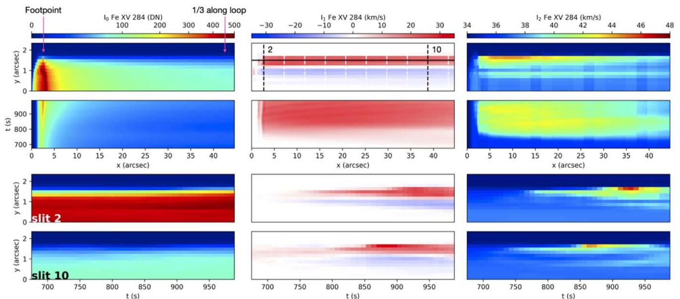
Figure 18. Short-term characteristics of MUSE synthetic observables (top view; see Figure 15) for a simulation modeling a coronal loop undergoing an impulsively excited and vertically polarized kink oscillation ( Cip_waves ; see Section 2 and Appendix A). The panel configuration, distance and time axis, LOS view, and exposure time are the same as in Figure 17 for the curved loop. Here we show the Fe XV 284 Å synthesis for the first one-third of the curved loop, focusing on a 5 minute interval during which the KHI develops. The top row shows a snapshot at t = 950 s, at the end of this stage. The KHI leads to steady upflows (blueshifts)/downflows (redshifts) with increased line widths at the loop boundary all along the loop (slits 2 and 10). Count rates are calculated as described in Appendix B.
