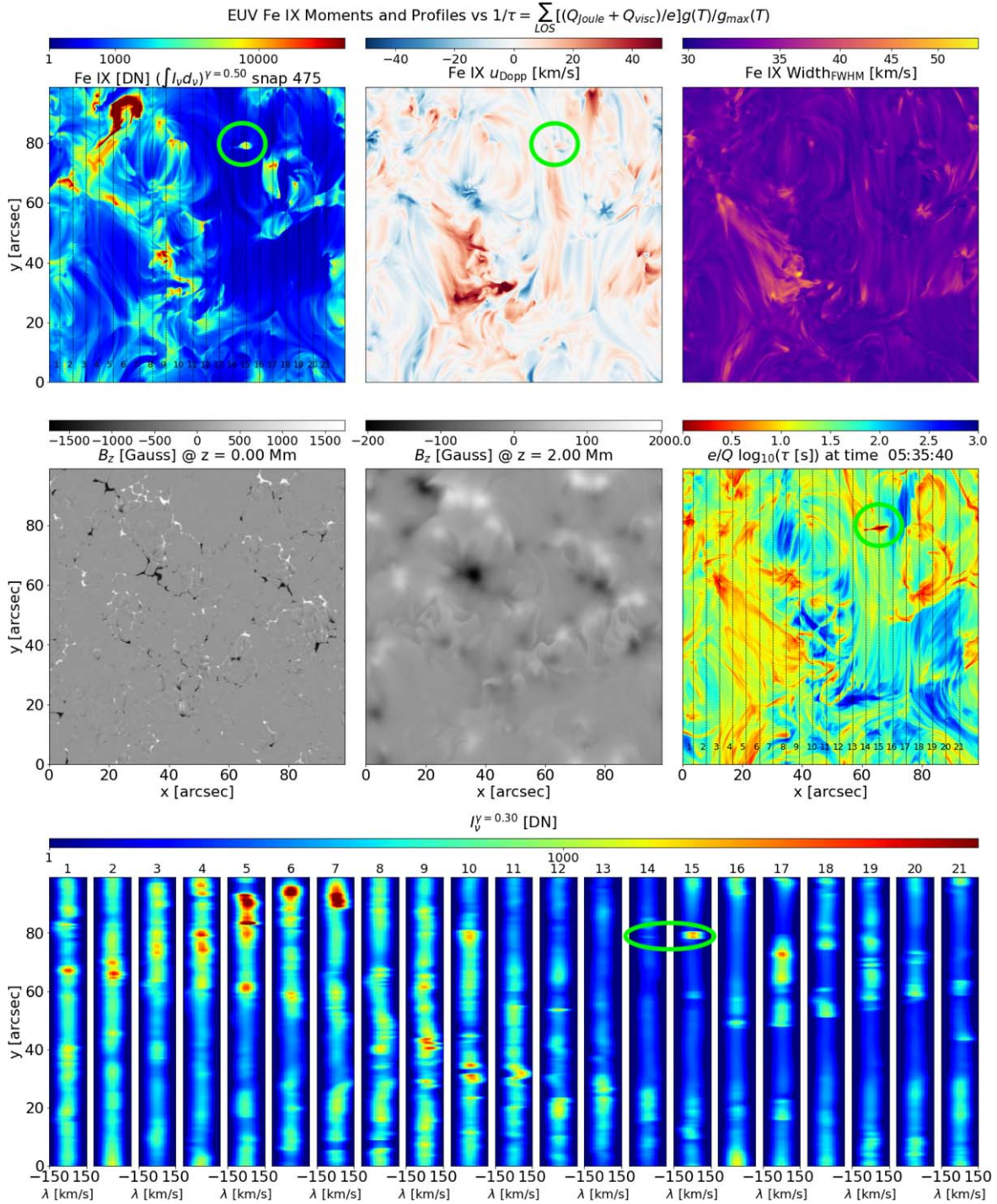
Figure 4. MUSE synthetic observables, from Bifrost 3D MHD model B_{\text{nw072100}} (see Table 2 and Appendix A), diagnosing heating through braiding. The upper three panels show the intensity, line shift, and line width of the Fe IX 171 Å line, while the second row of panels shows the photospheric field, the field 2 Mm above the photosphere, and a measure of the heating rate in the temperature range where this line is formed: (Q_{\text{Joule}} + Q_{\text{visc}})/e \times G(T)/G_{\text{max}}(T) , filtered over the normalized G(T) for the line in question and summed over the line of sight. The upper-left and lower-right panels also show the potential location of 21 of the 37 MUSE slits for a “sit-and-stare” observation. The bottom row of panels shows the line profiles of the Fe IX line at these locations. Braiding events occur throughout the simulated region as the magnetic field is driven by photospheric motions. Particularly strong heating is found in a small region near the top of the domain where x \sim [20, 40] and y \sim [85, 95] and along a diagonal that stretches from (x, y) \approx (15'', 60'') to (x, y) \approx (40'', 50'') , which outlines a long current sheet that shows continual episodic heating events. Note that the Fe IX line width responds strongly to these heating events all along the current sheet. Nanojets caused by reconnection resulting from braiding can also be found throughout this simulation. An example is shown in the green circles in the two left panels of the top row, and the right panel of the middle row. The assumed exposure time is 1.5 s. Count rates are calculated as described in Appendix B. An animated version of this figure is available and shows the spatiotemporal coherence of heating patterns caused by braiding and their effects on the MUSE observables, as described above. The animated version also includes the time series of the Fe XV and Fe XIX spectral bands.
