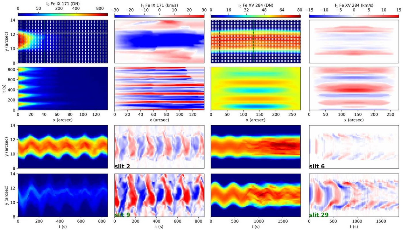
Figure 16. The comparison of MUSE observables predicted from two models of oscillating loops shows clear detectable differences between the continuously driven (PL_waves) and the impulsively driven (Cip_waves) cases, providing clear diagnostics for distinction. We show the zeroth (first and third columns) and first moment (second and fourth columns) for MUSE Fe IX 171 Å (model PL_waves, left two columns) and Fe XV 284 Å (model Cip_waves, right two columns). The x coordinate is along the loops, and we show half the loop for model PL_waves (footpoint located on the right end of the x -axis), and the full loop for model Cip_waves (footpoints located at the two extremes of the x -axis). The LOS corresponds to the face view (see Figure 15) but is at a 45^\circ inclination with respect to the kink oscillation direction. The integration times are 1.5 s and 5 s for the PL_waves and Cip_waves models, respectively. The top panels show the loops at a time when the KHI is already well developed, while the second row of panels tracks the evolution of the oscillation along the boundary of each loop. Note here that due to gravitational stratification and the mixing of plasma due to the KHI, only the loop footpoint is visible for model PL_waves (also see Karamelas et al. 2019b). The two bottom rows show time–distance maps for the zeroth and first moments, at two different heights (and slits, counting from left to right) along the loops. Note the increase in amplitude with height for the first moment, with the herringbone patterns and small-scale structure best visible toward the apex. Note also the damping of the oscillatory motion in the zeroth moment and decrease/increase in the first moment at the loop core/boundary due to resonant absorption, only visible in the impulsively driven model. Count rates are calculated as described in Appendix B. An animation of this figure is available. It shows the difference in the spatiotemporal patterns of the oscillatory signals between both models and the formation of the KHI, as illustrated in the figure and described in the text. (An animation of this figure is available.)
