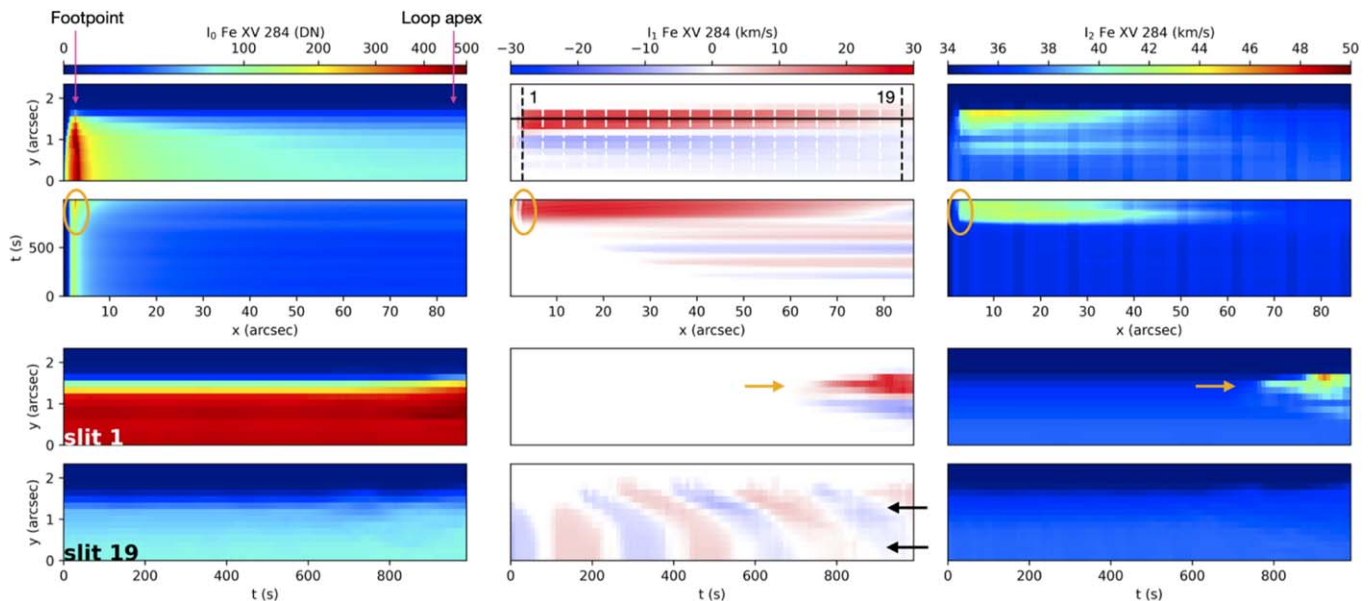
Figure 17. Long-term characteristics of MUSE synthetic observables (top view; see Figure 15) for a simulation modeling a coronal loop undergoing an impulsively excited and vertically polarized kink oscillation ( Cip_waves ; see Table 2 and Appendix A). The loop coordinate axis is transformed onto a curved trajectory to mimic a semicircular coronal loop (as in the RADYN models of Figure 11). Here we show the Fe XV 284 Å synthesis for half of the loop with a time integration of 5 s, with x = 0 (and slit 2) near the left footpoint and larger x (higher slit number) corresponding to rays crossing the loop higher up in the corona, up to the loop apex. The top row shows a snapshot at t = 950 s when the KHI is fully developed across the loop. The second row shows the time–distance maps of the moments, at the boundary of the loop (marked by the horizontal black line in the top middle panel). Note the distinct change in the first and second moments at t \approx 700 s, indicating the onset of the KHI. An increase in the intensity at the footpoints is marked with an orange circle. The two bottom rows show time–distance maps of the Fe XV moments, for two slits at different heights along the loops: slit 1 is at the footpoint, while slit 19 is at the apex (half of the loop). The black arrows mark the kink-mode attenuation and accompanied amplitude increase of the Alfvén waves at the boundary due to resonant absorption. The orange arrows mark the KHI onset. Count rates are calculated as described in Appendix B.
