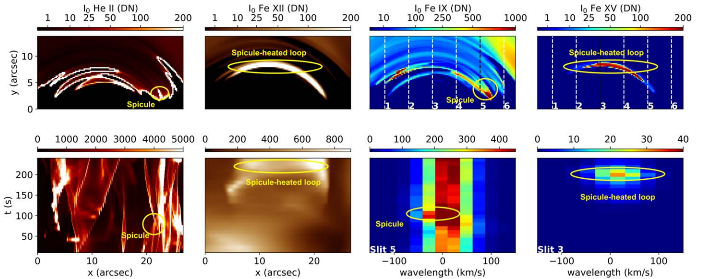
Figure 3. MUSE synthetic observables for a 2.5D Bifrost model ( B_en096014_gol ; see Table 2, Appendix A, and Figure 2) producing spicules and associated coronal heating. The top row shows side views (i.e., as seen at the limb) of the intensity at t = 240 s, from left to right, in the two MUSE CI passbands (He II 304 Å and Fe XII 195 Å), the MUSE SG lines (Fe IX 171 Å and Fe XV 284 Å). The second row shows the top view (i.e., as seen on disk) of the spacetime intensity maps in the two MUSE CI passbands (He II 304 Å and Fe XII 195 Å) in the left two panels. The right panels show the temporal evolution of the MUSE SG Fe IX and Fe XV spectra along slit 5 (at the footpoint, where the spicule occurs) and slit 3 (near loop top), respectively (see Figure 2). Time integration is 10 s for all Fe IX and for the limb view of Fe XV, and 20 s for Fe XV in the bottom-right panel. Count rates are calculated as described in Appendix B. The associated animation shows the time evolution of the temperature (top left) and velocity (bottom left) of the simulation, including the side view of the intensities shown in the top row of this figure (right four panels). An animation of this figure is available and shows the events circled in the figure during the temporal evolution of the spicule and subsequent coronal loop formation (as also described in the text).
