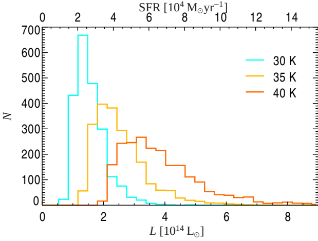
Fig. 17. Distribution of the FIR bolometric luminosity and SFR for three assumptions of the extragalactic dust temperature, T_{\text{xgal}} = 30, 35, \text{ and } 40 K.
