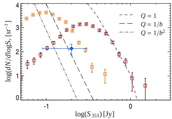
Fig. 19. PHZ number counts at 353 GHz (red squares), compared to the “clumps” number counts analytical predictions of Negrello et al. (2005) for three assumptions of the amplitude of the 3-point correlation function, Q , where b is the clustering bias parameter. Two cases of the PHZ number counts are presented, depending on the assumption made about the intrinsic number of clumps composing the PHZ source: n = 1 (red); and n = 3 (orange). The blue diamond gives the number counts estimate reported by Clements et al. (2014) for proto-cluster candidates selected from the Planck ERCSC catalogue.
