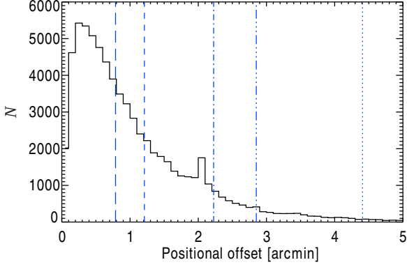
Fig. 7. Positional recovery. Histogram of the positional offsets between the centroid coordinates of the recovered sources and the initial coordinates. Vertical lines give levels of the maximum positional offset for the following lower percentiles: 50 % (long dashed); 68 % (dashed); 90 % (dash-dotted); 95 % (dash-dot-dot-dotted); and 99 % (dotted).
