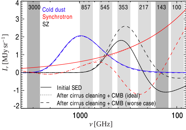
Fig. 6. Impact of the cleaning process on the SED of foreground astrophysical sources: cold Galactic sources (blue); SZ signal from galaxy clusters (black); and radio sources (red). The SEDs are shown before (solid line) and after cleaning, assuming two levels of CMB template quality, i.e., ideal (dotted line) or highly contaminated by extragalactic foregrounds at high \ell (dashed line).
