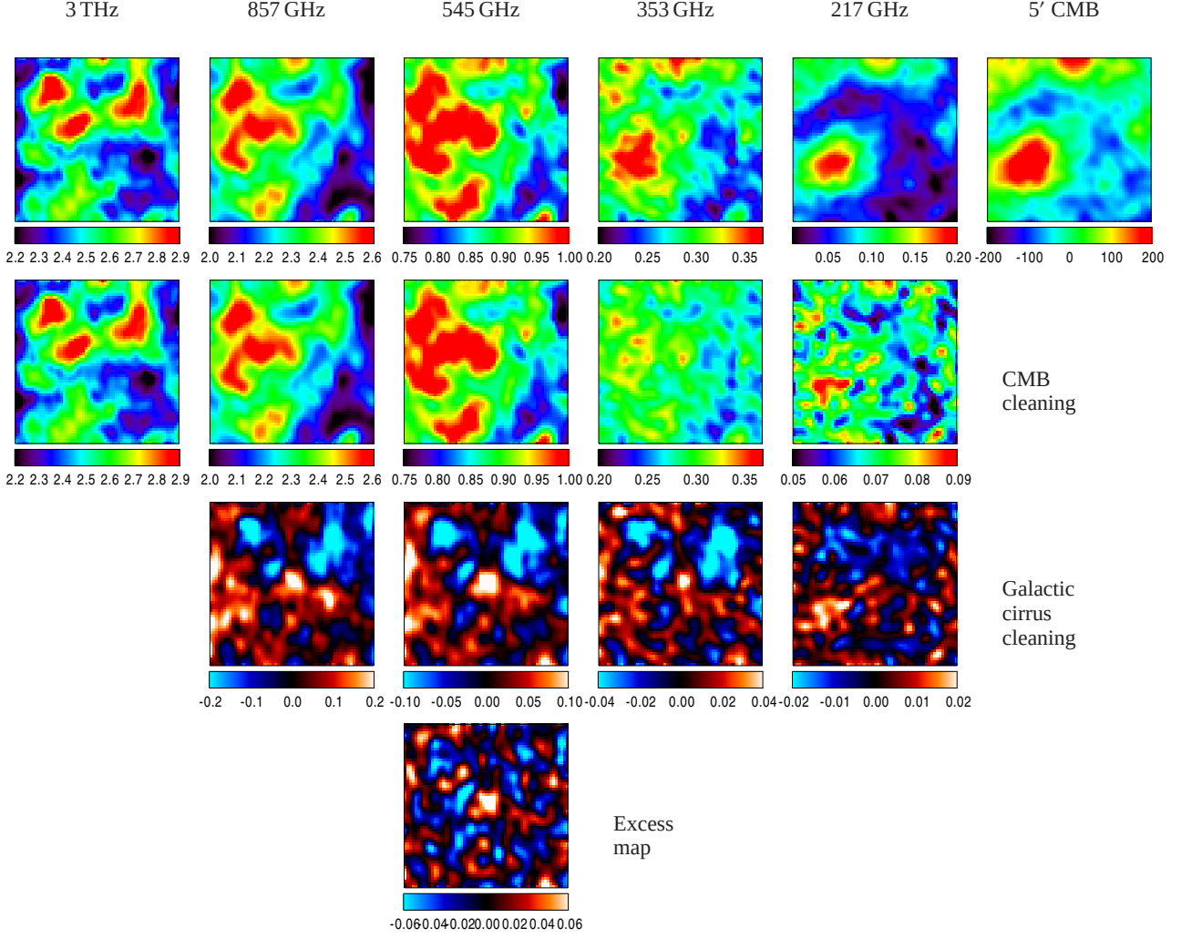
Fig. 3. Cutouts ( 1^\circ \times 1^\circ ) in Galactic coordinates of the IRIS and Planck maps centred on the source PHZ G095.50–61.59, after the various steps of the cleaning processing. First row: original maps at 5' plus the Planck 5' CMB template. Second row: maps after CMB cleaning. Third row: maps at 857, 545, 353, and 217 GHz after Galactic cirrus cleaning. Fourth row: excess map at 545 GHz. For the last two rows, the colour scale has been chosen so that positive residuals appear in red and negative residuals in blue. Units are expressed in \text{MJy sr}^{-1} , except for the CMB 5' template map, which is expressed in \mu\text{K}_{\text{CMB}} .
