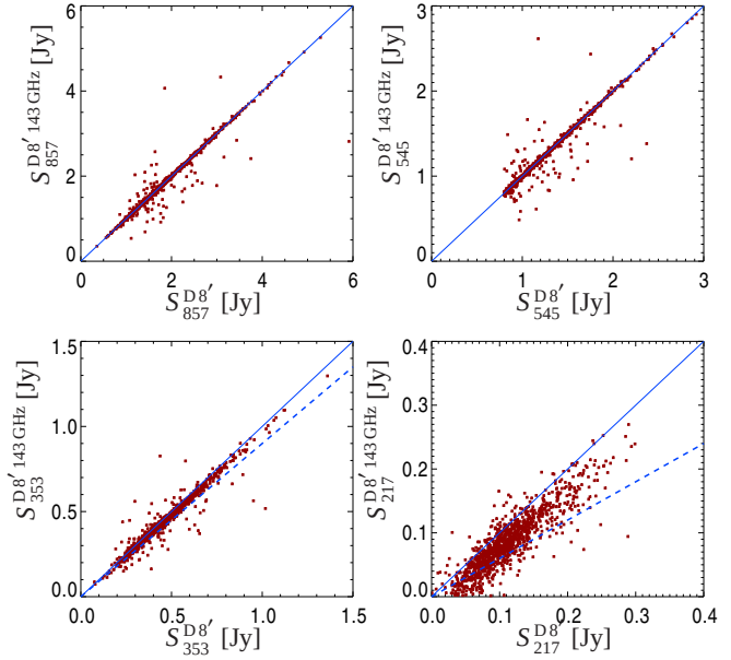
Fig. A.1. Comparison of the flux densities of the PHZ source candidates (at 8') computed on the cleaned maps obtained using the Planck 143 GHz map ( S_{\nu}^{D8' 143} ) or the SMICA CMB component map ( S_{\nu}^{D8'} ) as a CMB template during the cleaning processing. The blue line provides the 1:1 reference. The dashed line gives the expected attenuation coefficients of 10% at 353 GHz and 40% at 217 GHz due to extragalactic foreground contamination of the CMB template.
