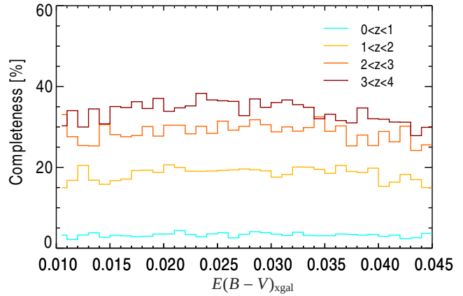
Fig. 12. Completeness as a function of extinction. This is shown for four bins of redshift: 0 < z < 1 (blue); 1 < z < 2 (yellow); 2 < z < 3 (orange); and 3 < z < 4 (brown). Only sources with input flux densities S_{545}^I > 0.5 Jy have been taken into account in this analysis.
