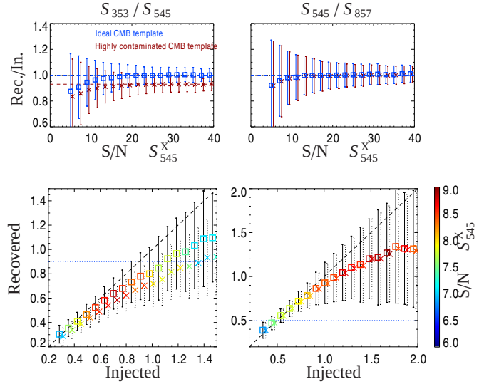
Fig. 10. Colour-colour ratio recovery. Left: S_{353}/S_{545} . Right: S_{545}/S_{857} . Top: ratio of recovered over injected colour-colour ratio (Rec./In.) as a function of the 545 GHz excess S/N. This is shown for two choices of the CMB template, i.e., ideal (blue squares) or highly contaminated by extragalactic foregrounds (red crosses). Bottom: recovered versus injected colour-colour ratio per bin of input colour-colour ratio. Again, two cases are shown depending on the quality of the CMB template, ideal (squares) or highly contaminated (crosses). The colour scale provides the average S/N of the 545 GHz excess inside each bin of input colour-colour ratio. The blue dotted lines show S_{353}/S_{545} < 0.9 and S_{545}/S_{857} > 0.5 , which are the colour criteria adopted for source selection.
