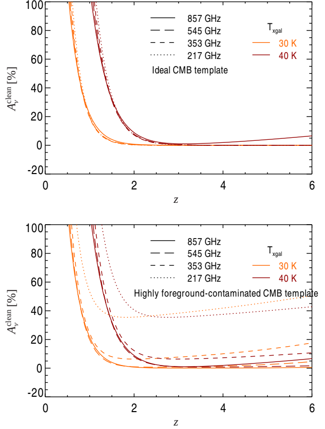
Fig. 5. Relative attenuation coefficient A_v^{\text{clean}} due to the cleaning process, as a function of redshift for each Planck -HFI band. This is computed for two input SEDs modelled by a modified blackbody ( T_{\text{xgal}} = 30 K and 40 K, with \beta_{\text{xgal}} = 1.5 ) embedded in foreground emission equally balanced between CIB and Galactic cirrus. It is shown for two extreme cases of the CMB template quality, i.e., ideal (upper panel) or highly contaminated by extragalactic foregrounds at high \ell (lower panel).
