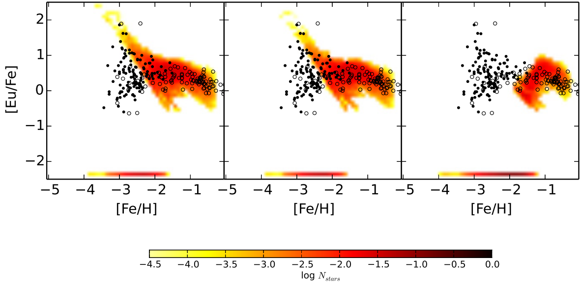
Fig. 1. Left panel: results for [\text{Eu}/\text{Fe}] vs. [\text{Fe}/\text{H}] for model NS00. This model has a delay time for the NSMs of 1 Myr, constant Eu production of 5 \times 10^{-6} M_{\odot} per merging event, and no Eu from SNeII. The density plot is the distribution of simulated long-living stars for our model (see the bar below the figure for the colour scale). The long-living stars formed without Eu (formally [\text{Eu}/\text{Fe}] = -\infty ) are shown at [\text{Eu}/\text{Fe}] = -2.4 . The model predictions are compared to data collected in Frebel (2010a) ; we show as black dots stars with [\text{C}/\text{Fe}] < 0.9 (to avoid binary enrichment), the open dots are stars with no carbon measurement. Central panel: same as left panel , but for model NS01. This model has a delay time for the NSMs of 10 Myr, constant Eu production of 5 \times 10^{-6} M_{\odot} per merging event, and no Eu from SNeII. Right panel: again same as for the left panel , but for model NS02. This model has a delay time for the NSMs of 100 Myr, constant Eu production of 5 \times 10^{-6} M_{\odot} per merging event, and no Eu from SNeII.
