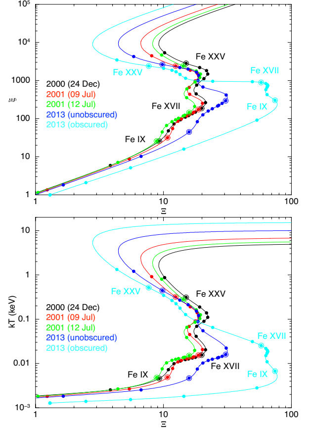
Fig. 13. Thermal stability curves for photoionised gas in NGC 5548, showing \xi plotted versus \Xi (top panel) and temperature kT plotted versus \Xi (bottom panel). They have been calculated for SEDs (displayed in Figs. 11 and 12) derived from our broadband modelling of the continuum as described in Sect. 6. The circles on the stability curves indicate the positions at which ionic column densities of Fe peak on the (\Xi, \xi) and (\Xi, T) phase space. To guide the eye, the location of Fe IX, Fe XVII, Fe XXV have been indicated with open circles around filled circles.
