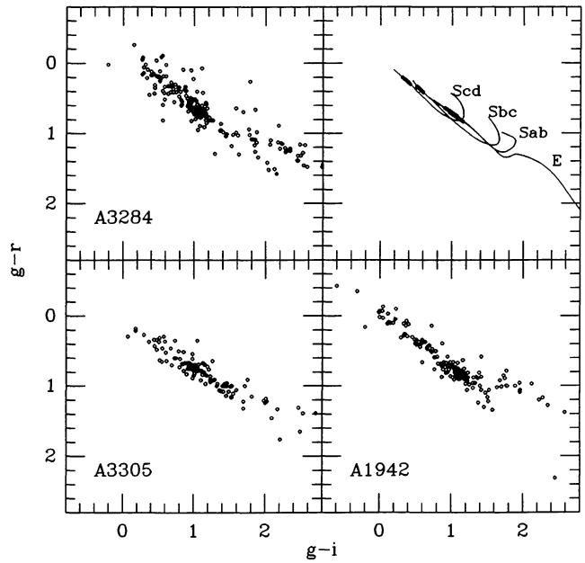
Fig. 11. Two-colour (g-r)/(g-i) diagrams for the complete photometry in the fields of the three clusters. Upper right panel shows the expected loci with increasing redshift from z=0 \rightarrow 1 (in the sense of increasing g-i ) for elliptical galaxies (E) and spirals of different types (Sab, Sbc, Scd). Boldface mark the expected colours in the range 0.15 < z < 0.22
