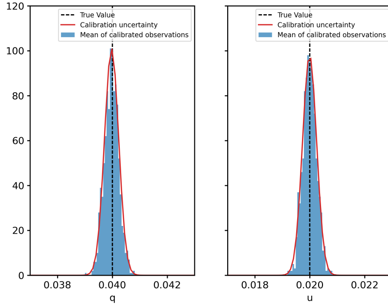
Figure 13. Distribution at 2.7 keV of the centers of observations (each consisting of 10^4 iterations of which each with 10^7 events) corrected with 10^3 different calibration measurements. The difference with the distribution of Fig. 12 is that this is a distribution of the centers of 10^3 distributions such as that of Fig. 12. The distribution is correctly centered on the true value, with a width given by the calibration uncertainty (2nd term of Eq. 41).
