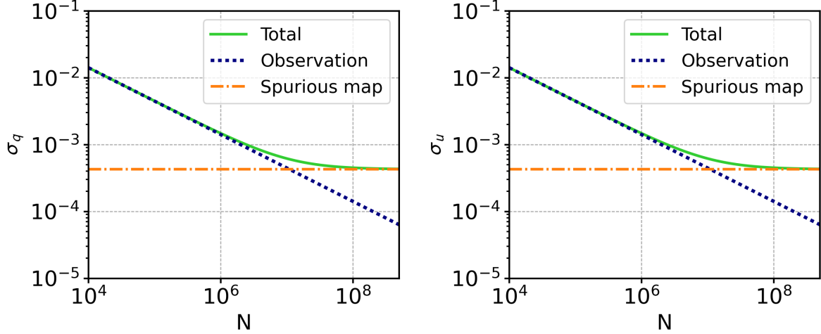
Figure 5. Comparison of the 1st term (Observation) and 2nd term (Spurious map) of the uncertainty expression (Eq. 41) as a function of the number of events of the observation. It can be seen that the 2nd term is often negligible. Also plotted is the total quadratic sum of the two terms, that tends to an asymptotic value which is the residual due only to calibration. This example is at 2.7 keV with 7 \cdot 10^6 events in the spurious modulation map.
