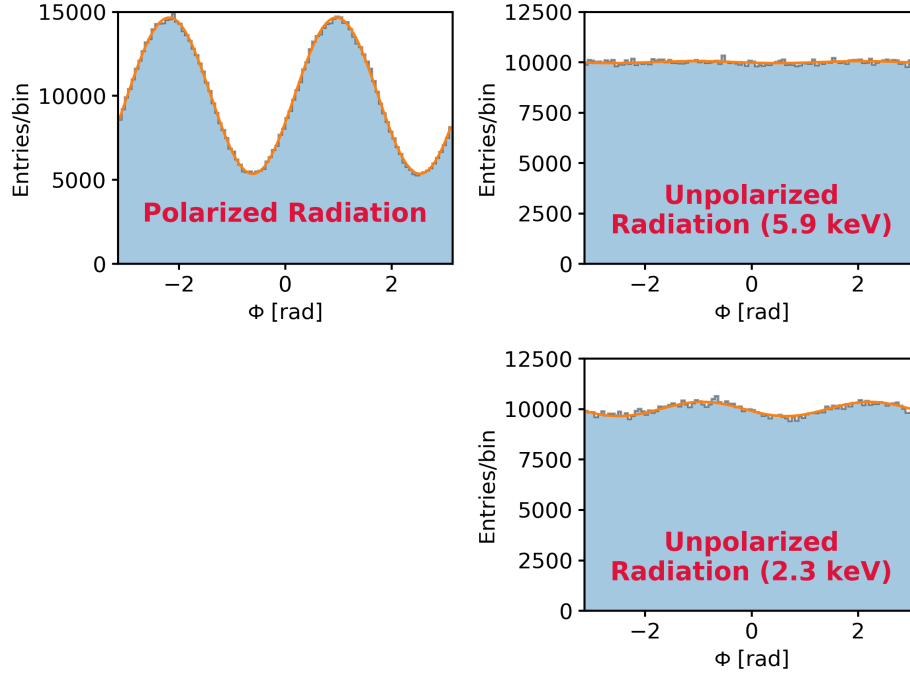
Figure 2. Modulation curves for polarized (left), unpolarized at 5.9 keV (upper right) and unpolarized at 2.3 keV (bottom right) radiation. For polarized radiation a modulation is seen, which is absent for unpolarized radiation at high energies, but reappears at low energies as spurious modulation.
