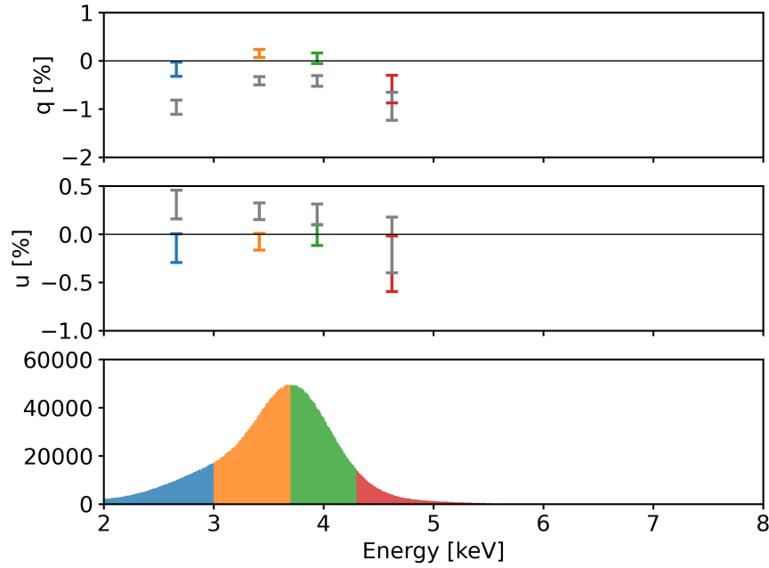
Figure 9. Spectra of the Ca X-ray tube with the modulation computed in energy bins. The colored points are corrected for spurious modulation using the photon by photon correction (therefore sensitive to the different energies), while the gray points are uncorrected. The corrected points are compatible with 0 as expected for the Ca X-ray tube, while for the uncorrected points the decreasing trend of spurious modulation with energy is evident.
