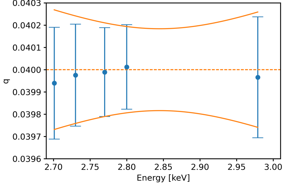
Figure 14. Centers and widths of Stokes parameter q (the u case is very similar) obtained from fitting the distributions of calibrations, such as the one in Fig. 13, at different energies. The orange lines are the widths computed with Eq. 42, centered on the true value (dashed line). The reason for the decrease in width is that the values in-between calibration energies are linearly interpolated, and the weighted combination of Eq. 42 is more likely to be close to the center if far away from the calibration energies.
