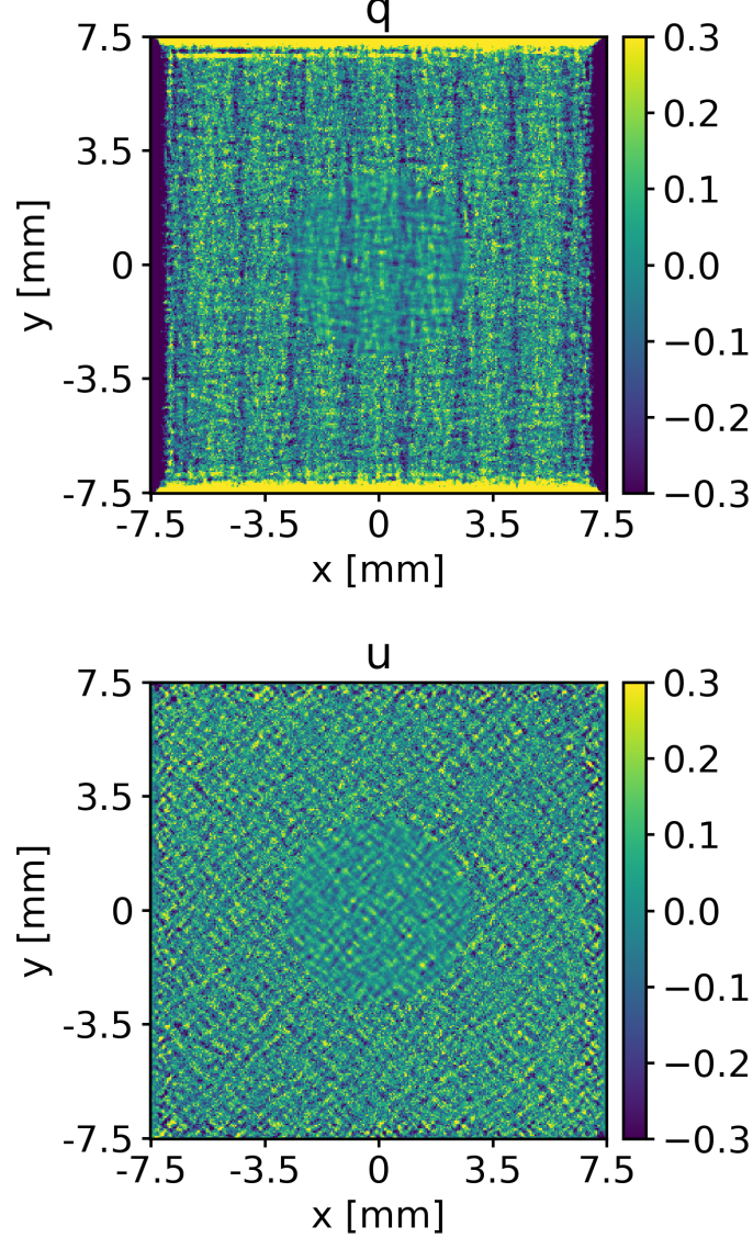
Figure 4. Example of spurious modulation maps for Stokes parameters q and u at 2.7 keV. The central region is smoother because it was calibrated with a larger statistics. It is also worth noting that values at the border are biased because photoelectric tracks are truncated by the physical size of the ASIC used for reading out the signal. The bias is such that the angle is biased to 90^\circ for vertical edges and to 0^\circ for horizontal edges. q is defined as the cosine of twice such angle (Eq. 2) and, therefore, values are biased to \sim \cos(2 \cdot 90^\circ) and \sim \cos(2 \cdot 0^\circ) . u (Eq. 3), instead, is \sim \sin(2 \cdot 90^\circ) and \sim \sin(2 \cdot 0^\circ) and therefore the bias is around 0.
