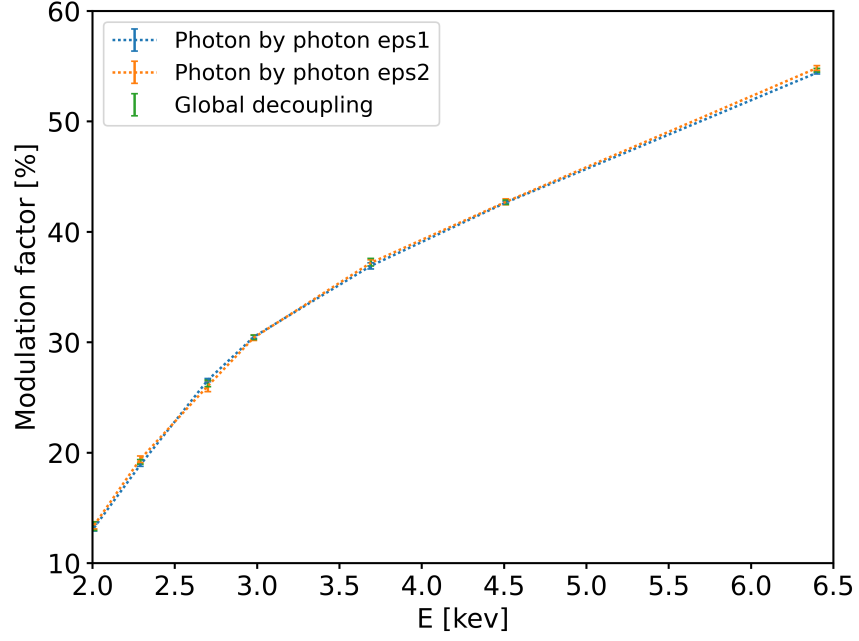
Figure 8. Same as Fig. 7 but for the modulation factor (obtained by dividing the source modulation of the polarized measurements by the source polarization, as in Eq. 1).
