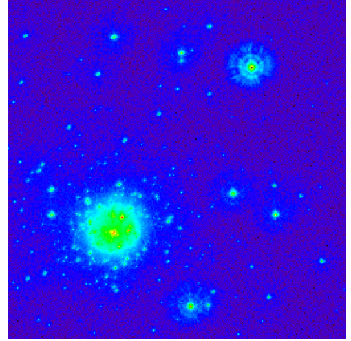
Fig. 1. Simulation of an observation of a star cluster through HST before COSTAR correction.
