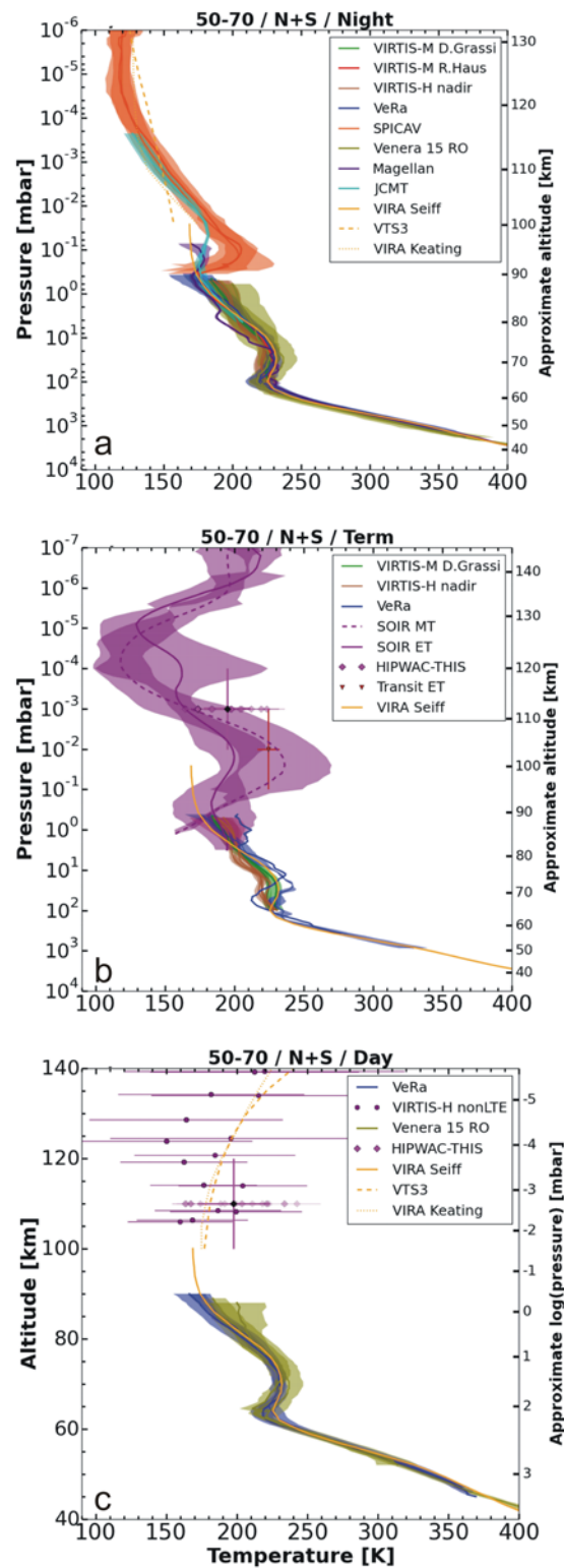
Figure 18: same as Figure 16 but for combined temperature profiles from the Northern and Southern hemispheres between 50° and 70° latitude. Panel (a): night side, panel (b): terminators, panel (c) day side.
