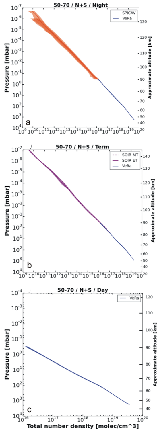
100 Figure 23: same as Figure 21 but for the latitude bin 50° to 70°. Panel (a): night side, panel (b): 101 terminator zones, panel (c): day side. The colored areas mark the one standard deviation uncertainty of 102 the average profiles for each experiment. Approximate altitudes are shown on the right hand vertical 103 axis.
