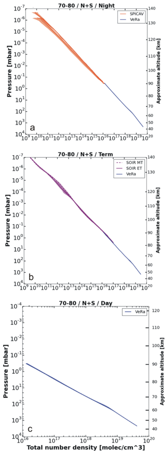
Figure 24: same as Figure 21 but for the latitude bin 70° to 80°. Panel (a): night side, panel (b): terminator zones, panel (c): day side. The colored areas mark the one standard deviation uncertainty of the average profiles for each experiment. Approximate altitudes are shown on the right hand vertical axis.
