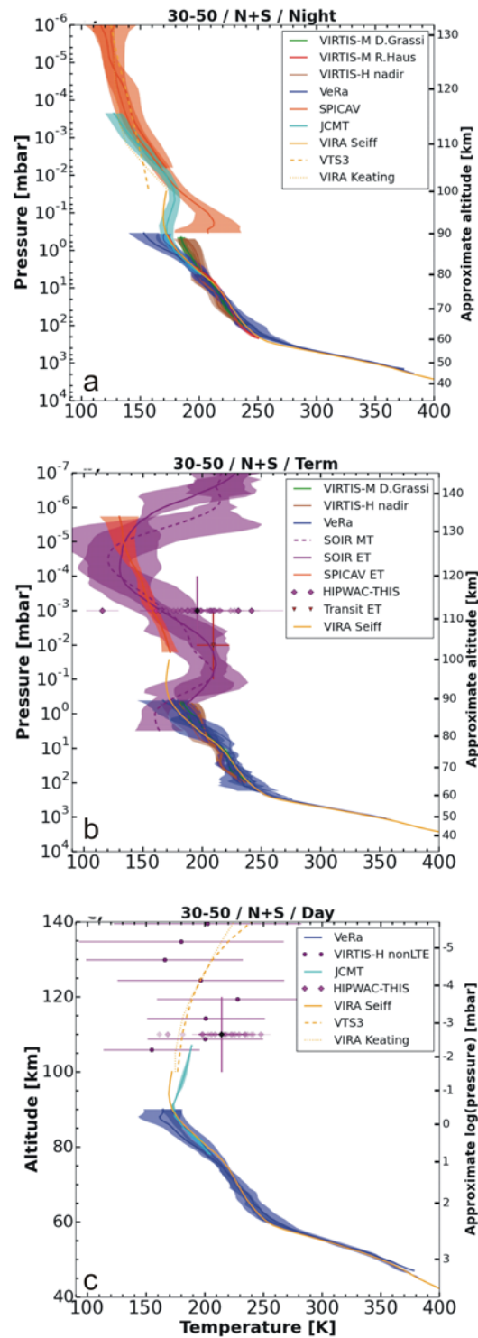
Figure 17: same as Figure 16 but for combined temperature profiles from the Northern and Southern hemispheres between 30° and 50° latitude. Panel (a): night side, panel (b): terminators, panel (c) day side.
