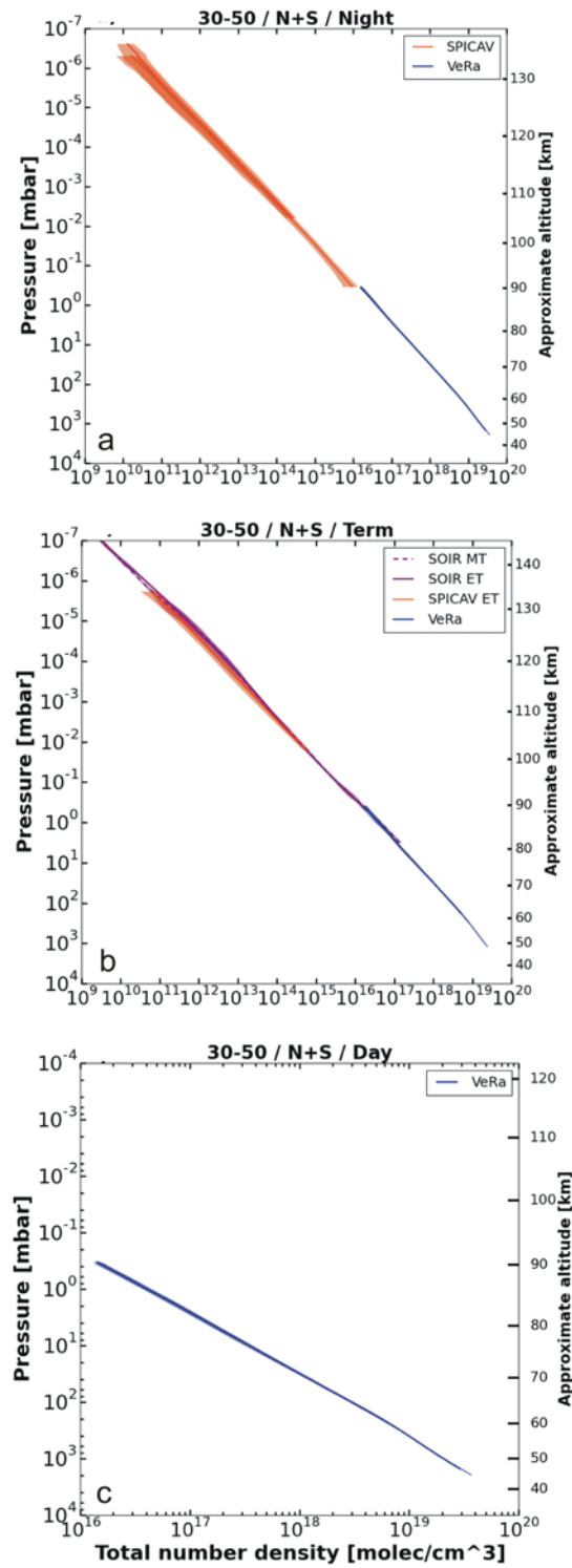
Figure 22: same as Figure 21 but for the latitude bin 30° to 50°. Panel (a): night side, panel (b): terminator zones, panel (c): day side. The colored areas mark the one standard deviation uncertainty of the average profiles for each experiment. Approximate altitudes are shown on the right hand vertical axis.
