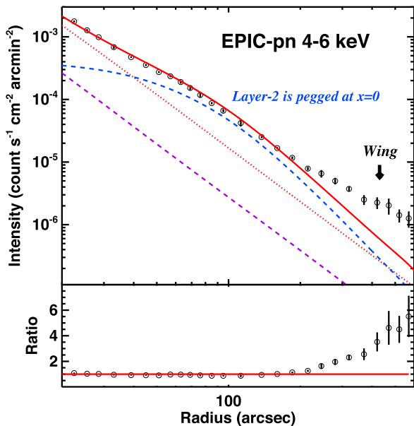
Figure 8. Radial profile observed by XMM-Newton EPIC-pn in the 4–6 keV band, overplotted with the EPIC-pn PSF (red dotted curve), dust layer-1 (magenta dashed curve), layer-2 whose fractional distance is pegged at 0 and fractional width pegged at the lower limit of 0.01 (blue dashed curve), and the total model (red solid curve). A significant excess flux exists outside 200 arcsec, which cannot be fitted by any dust model (black arrow).
