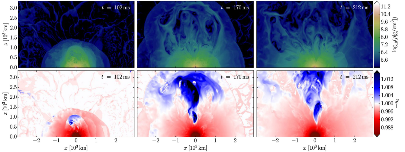
Figure 1. Meridional view of rest-mass density (top) and -u_t (bottom) at 102, 170, and 212 ms after merger for model ‘B5e15’. Blue (red) colour in the bottom row corresponds to fluid elements that are unbound (bound) according to the geodesic criterion (see e.g. Hotokezaka et al. 2013 for u_t definition).
