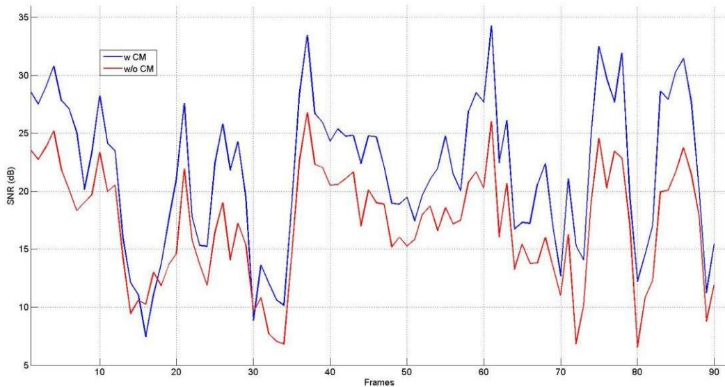
Fig. 5. SNR behavior, for 3 MHz, connected to the radargrams of Fig. 3. The blue and the red lines show the SNR obtained with and without the CM respectively.
