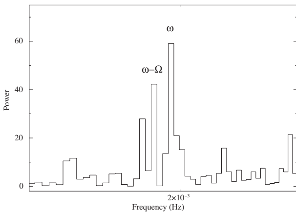
Figure 2. PN 0.3–12 power spectrum zoomed in the spin, \omega , 0.00196 Hz, and beat (\omega - \Omega) , 0.00190 Hz, frequency region.
