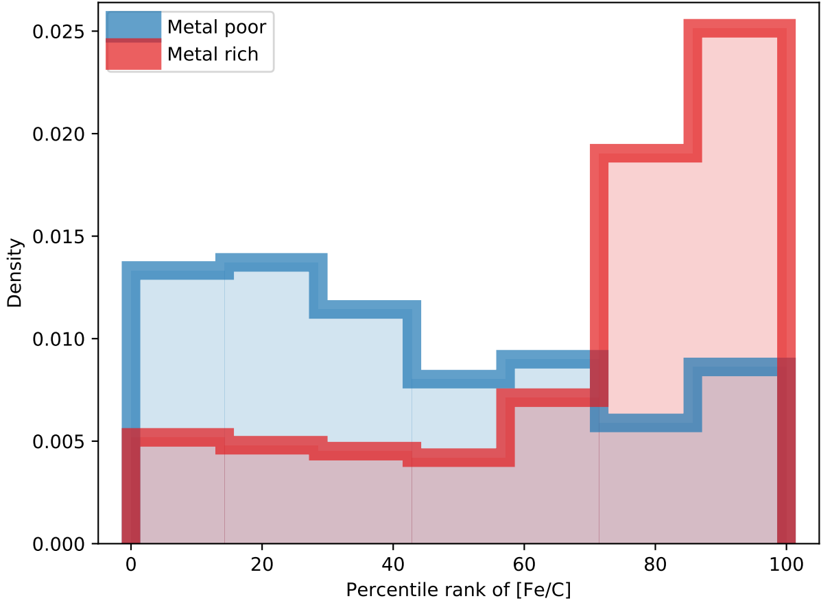
Figure 2: The [\text{Fe}/\text{C}] percentile ranks. The plot shows the distribution of [\text{Fe}/\text{C}] percentile ranks for the metal-rich (red histogram) and metal-poor (blue histogram) components of chemically anomalous pairs. The high [\text{Fe}/\text{C}] percentile ranks characteristic of the metal-rich components indicate that these stars have [\text{Fe}/\text{C}] ratios that are typically larger than the values seen in solar twin stars.
