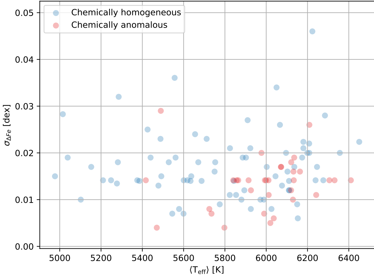
Figure 4: The \sigma_{\Delta Fe} - \langle T_{eff} \rangle diagram. The figure shows the uncertainty associated to the differential iron abundance \sigma_{\Delta Fe} as a function of the average temperature of the two binary components \langle T_{eff} \rangle . The chemically homogeneous pairs are shown in blue, while the chemically anomalous are in red.
