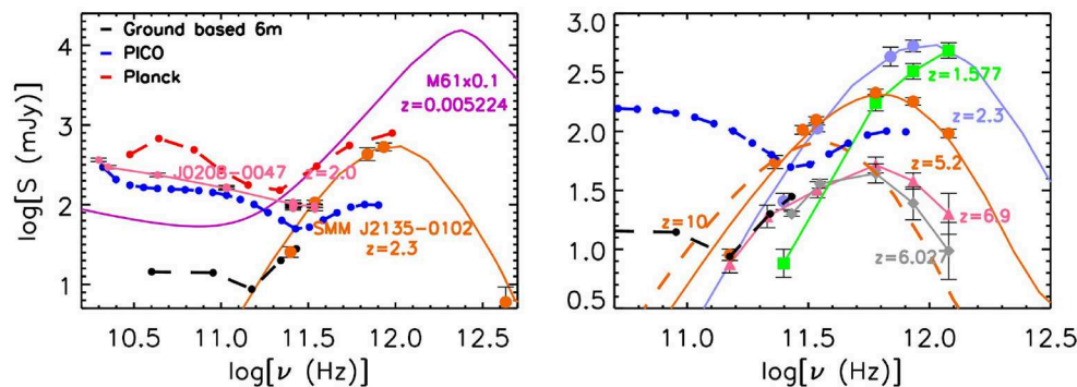
FIGURE 2 | Spectral energy distributions of extragalactic sources in the frequency range of CMB experiments, compared with the estimated detection limits of the PICO project and with the completeness limits of the SPT surveys extrapolated to 40 and to 270 GHz, to cover the range of the CMB-S4 project. The PCCS2 90% completeness limits in the “extragalactic zone” are also shown for comparison (in the left panel only). At wavelengths shorter than a few mm the dominant extragalactic population are dusty star-forming galaxies. At longer wavelengths radio sources, mostly blazars, take over. The spectral energy distributions (SEDs) of blazars are characterized by a relatively flat continuum spectrum exemplified by that of J0208-0047 at z \simeq 2.0 (flat solid orange line). Dusty star-forming galaxies are a mixture of local and high- z strongly gravitationally lensed objects. Local galaxies are, by far, the brightest extragalactic sources at sub-mm wavelengths. Their SEDs are exemplified by that of the dusty star-forming galaxy M61, scaled down by a factor of 10. Some examples of SEDs of strongly lensed galaxies are shown: SDP 9 ( z = 1.577 ; Negrello et al., 2010), SMMJ2135-0102 ( z = 2.3259 ; Swinbank et al., 2010), HLS J091828.6+514223 ( z = 5.2 ; Combes et al., 2012), HATLAS J090045.4+004125 ( z = 6.027 ; Zavala et al., 2018), and SPT-S J031132-5823.4 ( z = 6.9 ; Strandet et al., 2017). The dashed orange SED represents that of HLS J091828.6+514223 scaled to z = 10 to show that galaxies like it are visible up to very high redshifts both by ground-based and by space-borne next generation CMB experiments.
