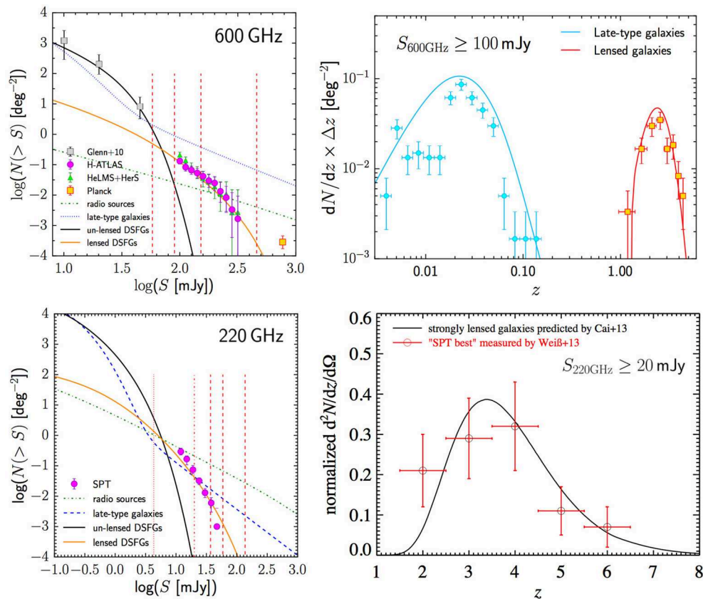
FIGURE 3 | (Upper left panel) Integral counts of strongly lensed galaxies from Herschel surveys at 500 \mu\text{m} (600 GHz; green and magenta data points from Negrello et al., 2017a), compared with the predictions of the Cai et al. (2013) model (solid orange line). The yellow square on the bottom-right corner is our own estimate of the counts of strongly lensed galaxies detected by Planck . The counts of unlensed proto-spheroidal galaxies (data points from Glenn et al., 2010, black squares; model by Cai et al., 2013, solid black line), of radio sources (dotted green line, model by Tucci et al., 2011) and of normal and starburst late-type galaxies (dotted blue line, model by Cai et al., 2013) are also shown for comparison. The vertical dashed orange lines show, from right to left, the 90% completeness limit of the PCCS2 and the 5\sigma detection limits for space-borne CMB experiments with 1, 1.5 and 2 m telescopes working at the diffraction limit. This panel shows a modified version of Figure 8 of Negrello et al. (2017a). (Upper right panel) Redshift distribution of galaxies brighter than 100 mJy at 500 \mu\text{m} , derived from the full H-ATLAS catalog (data points with Poisson errors) compared with the predictions of the Cai et al. (2013) model (solid lines). There is a clear bimodality. On one side we have nearby late-type galaxies, almost all at z \leq 0.06 , and hence easily recognizable in optical/near-infrared catalogs. On the other side we have dust enshrouded, hence optically very faint, gravitationally lensed galaxies at z \geq 1 and up to z > 4 . (Lower left panel) Integral counts of strongly lensed galaxies from the SPT survey at 220 GHz (1.4 mm; magenta data points; Vieira et al., 2010) compared with the prediction of the Cai et al. (2013, orange solid line) model. Counts of radio sources and of late-type galaxies are from the same models as in the upper panel. The vertical lines show, from right to left, the 5\sigma detection limits for diffraction limited 1, 1.5, and 2 m telescopes, the completeness limit of the SPT survey (Mocanu et al., 2013) and the 5\sigma confusion limit for a 6 m telescope. (Lower right panel) Estimated redshift distribution of strongly lensed galaxies with S_{220\text{GHz}} > 20 \text{ mJy} (Weiß et al., 2013) compared with the prediction of the Cai et al. (2013) model.
