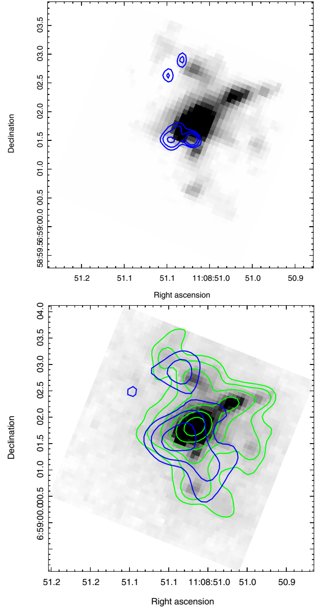
Fig. 4. HST U -band image of J1108+0659 overplot with the 8.5 GHz VLA image ( upper panel , HST in greys and VLA in contours) and with the 5.0 GHz VLA image ( lower panel , HST in greys and green contours and VLA in blue contours). The overplot with the 8.5 GHz radio image shows the slight offset between the candidate radio core and the north-west core detected in the UV continuum. The south-east core is undetected in the UV continuum. The overplot with the 5.0 GHz radio image clearly shows that the extended radio emission and the UV continuum are co-spatial.
