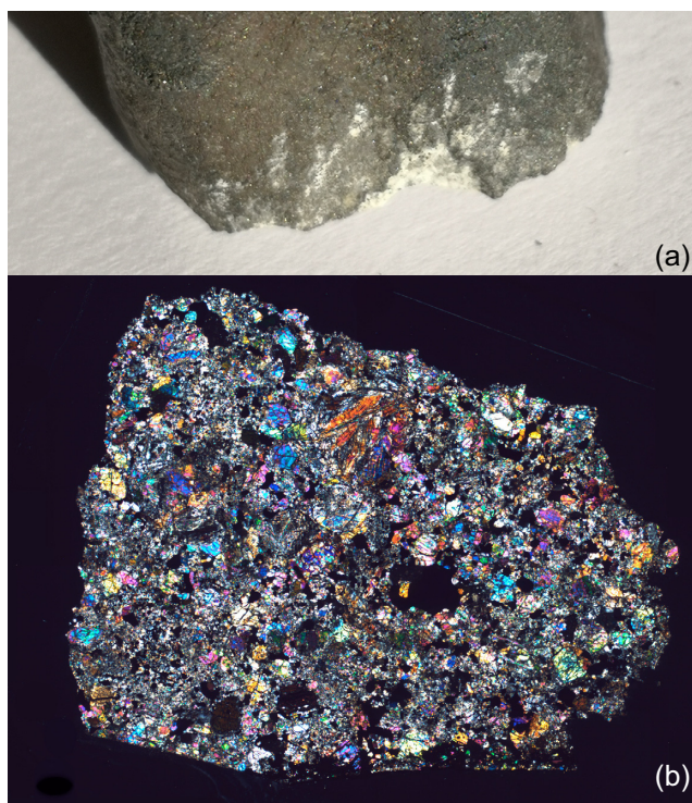
Figure 2. Details of the larger fragment F2 of the Cavezzo meteorite. (a) White streaks occur on one edge of F2, suggesting on-ground breakup of the original body; (b) photomosaic of polarizing optical microscope images (transmitted light, crossed polars) of a thin sections obtained from F2 (field width 12 mm) showing chondrules and chondrule fragments distributed in the matrix.
