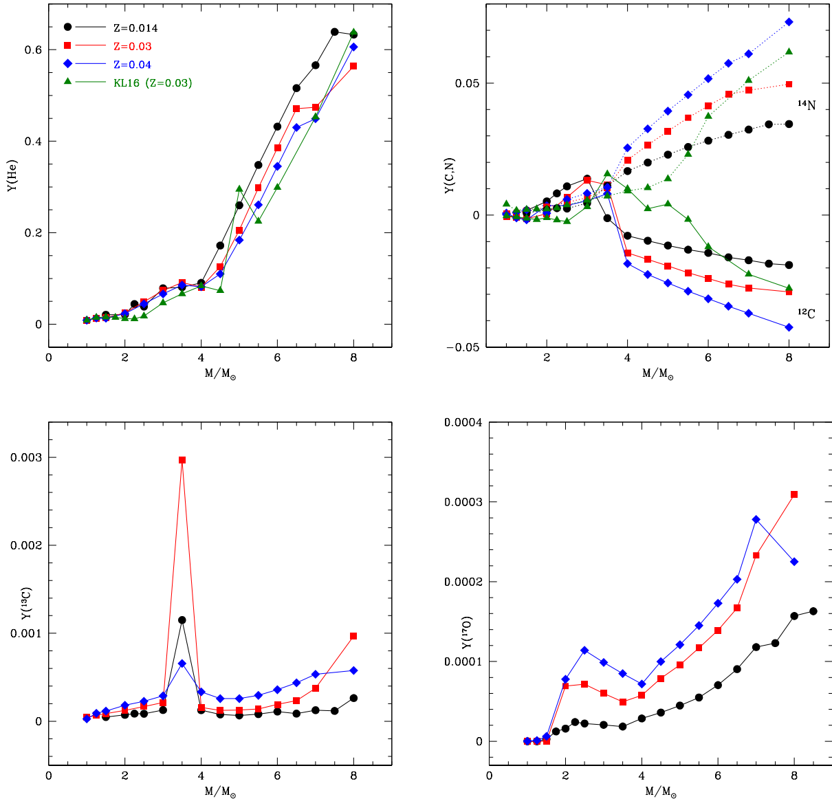
Fig. 8. Yields in solar masses of helium ( top-left panel ), ^{12}\text{C} and ^{14}\text{N} ( top, right ), ^{13}\text{C} ( bottom, left ), and ^{17}\text{O} ( bottom, right ) of our Z = 0.03 (red squares) and Z = 0.04 (blue diamond) AGB models and of solar-metallicity models by Ventura et al. (2018). Green triangles indicate the helium, carbon, and nitrogen yields published in Karakas & Lugaro (2016).
