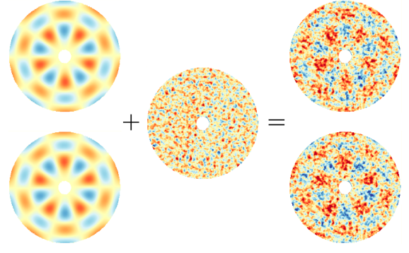
Fig. 1. Example of the phase used to run a single step of the push-pull calibration with partial correction (for the 8m-class telescope case and 0.2 m sup-aperture size): on the left part mode no. 50 of the modal base with positive (top, push) and negative (bottom, pull) sign, on the central part a random realization of the partial correction (i.e., turbulence residual), and on the right part the combination of mode and partial correction. The wavefront root mean square (RMS) of the mode is 40nm and the wavefront RMS of the random realization of the partial correction is 46nm (corresponding to the residual correction level expected for a seeing of 0.4arcsec). We note that these RMS values are selected for display purpose, in general, the amplitude of the push-pull (i.e., the wavefront RMS of the mode) is much smaller than the RMS of the partial correction.
