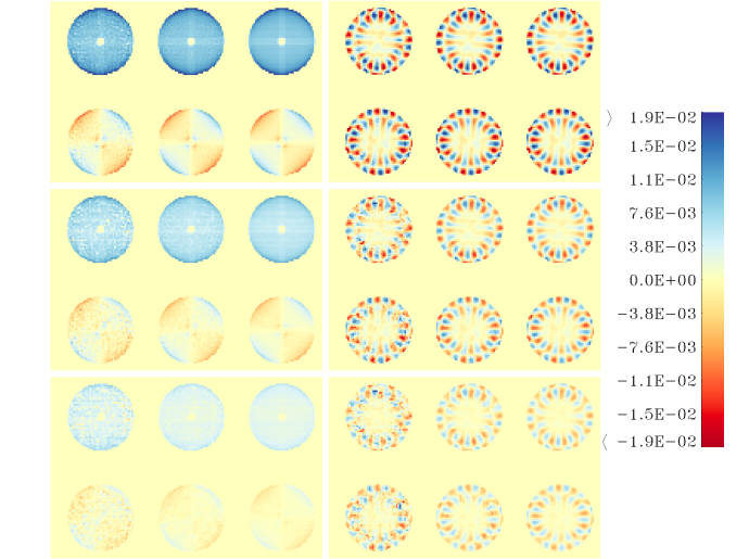
Fig. 2. Tip (left) and mode no. 100 (right) signals (x and y) from interaction matrices with different numbers of partial correction realizations (from left to right): 1, 8, and 70. Top: Partial correction for a seeing of 0.4arcsec, middle, partial correction for a seeing of 0.8arcsec, bottom, partial correction for a seeing of 1.2arcsec. Note: the signals amplitude is reduced when seeing increases. Refers to the sub-aperture size of 0.2 m. 8m-class telescope case.
