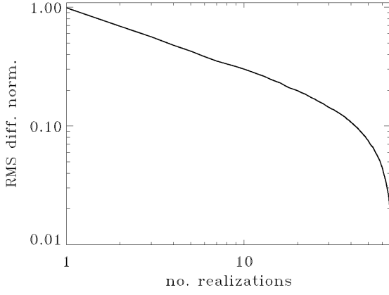
Fig. 3. RMS of the difference between the IM computed with x+1 and x realizations of partial correction normalized by the RMS of the IM computed with N=70 realizations. Seeing is 1.4 arcsec and sub-aperture size is 0.2 m for the 8m-class telescope case.
